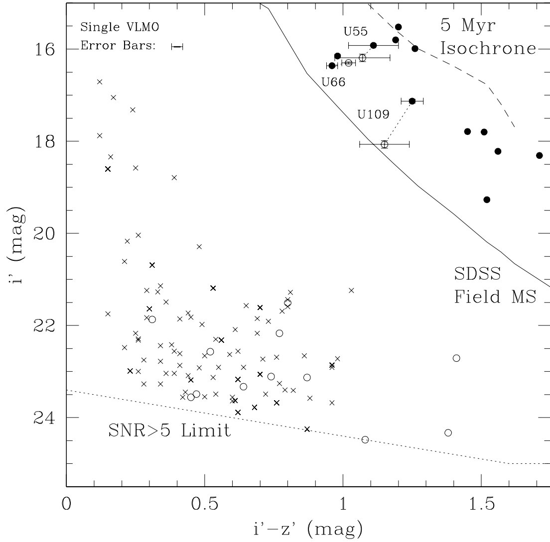
FIG. 3.— An i' vs i' - z' color magnitude diagram. Primary Upper Sco targets are shown as filled circles, neighbors within 5'' are shown as open circles, and widely-separated objects are shown as crosses. The SDSS field main sequence (solid line), a 5 Myr isochrone (dashed line), and the detection limits of the survey (dotted line) are also shown. Candidate binary VLMO pairs are connected with dotted lines and labeled. The error bars for binary components are associated with each point, and the error bars for single objects are shown in the upper left corner.
