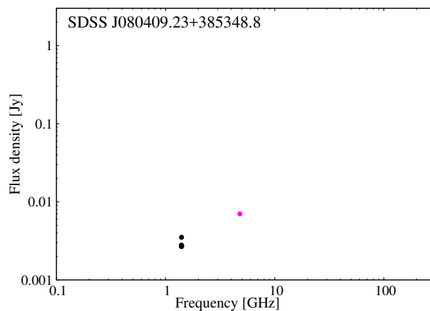
Fig. A.28. Radio spectrum of J080409.23+385. Only detections. Colours as in Fig. A.25.
