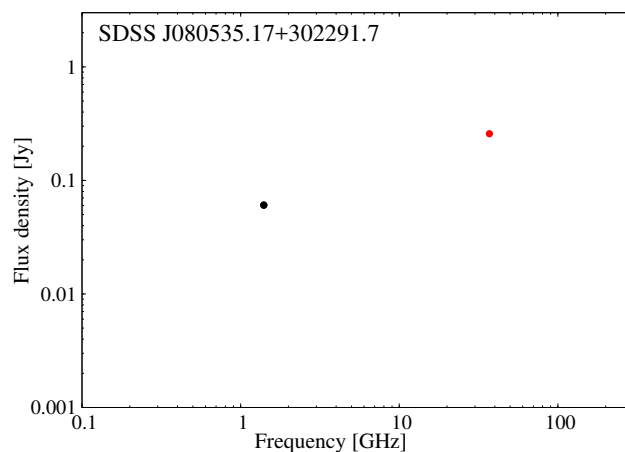
Fig. A.29. Radio spectrum of J080535.17+302. Only detections. Colours as in Fig. A.25.
