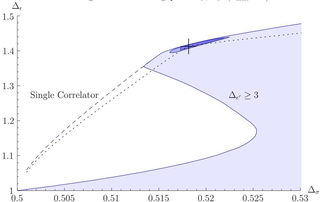
Figure 3: Allowed regions in a \mathbb{Z}_2 -symmetric \text{CFT}_3 , assuming various gaps in the scalar spectrum. The dashed line is an upper bound on \Delta_\epsilon using crossing symmetry and unitarity of \langle \sigma\sigma\sigma\sigma \rangle , with no assumptions about gaps, at n_{\max} = 6 . The black dotted line is the same bound with n_{\max} = 10 . The light blue shaded region assumes a gap \Delta_{\epsilon'} \geq 3 in the \mathbb{Z}_2 -even sector. The medium blue shaded region assumes a gap \Delta_{\sigma'} \geq 3 in the \mathbb{Z}_2 -odd sector, and uses crossing symmetry for the system of correlators \langle \sigma\sigma\sigma\sigma \rangle, \langle \sigma\sigma\epsilon\epsilon \rangle, \langle \epsilon\epsilon\epsilon\epsilon \rangle (same as figure 2). The dark blue region assumes both \Delta_{\sigma'}, \Delta_{\epsilon'} \geq 3 , and uses the system of multiple correlators. All bounds other than the black dotted line are computed with n_{\max} = 6, \nu_{\max} = 8 (21 components for single correlator bounds, 105 components for multiple correlator bounds). The 3D Ising point is indicated with black crosshairs.
