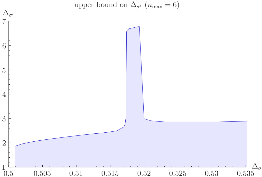
Figure 1: An upper bound on \Delta_{\sigma'} , where (\Delta_\sigma, \Delta_\epsilon) are constrained to lie on the n_{\max} = 10 single correlator bound (black dotted line in figures 3 and 4). The sharp spike in the bound occurs when the values of \Delta_\sigma, \Delta_\epsilon lie within the allowed region in figure 3, with no assumption about \mathbb{Z}_2 -even gaps (medium-blue shaded region). Only when \Delta_\sigma, \Delta_\epsilon take these values, is it possible to have \Delta_{\sigma'} \geq 3 , and indeed the upper bound on \Delta_{\sigma'} becomes extremely weak. This bound is computed at n_{\max} = 6, \nu_{\max} = 8 . We expect that as n_{\max} increases, it becomes more sharply peaked, while the top moves down to the correct value of \Delta_{\sigma'} in the 3D Ising model. At n_{\max} = 10, \nu_{\max} = 14 we have computed the stronger bound \Delta_{\sigma'} \leq 5.41(1) (the dashed line) at the points (\Delta_\sigma, \Delta_\epsilon) = (0.5181, 1.41206), (0.51815, 1.41267), (0.5182, 1.41312) .
