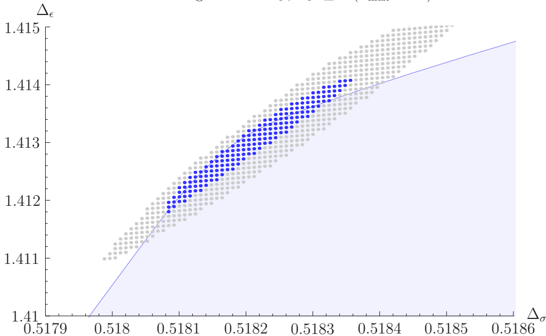
Figure 5: Allowed and disallowed (\Delta_\sigma, \Delta_\epsilon) points in a \mathbb{Z}_2 -symmetric \text{CFT}_3 with only one relevant \mathbb{Z}_2 -odd and \mathbb{Z}_2 -even scalar, using the constraints of crossing symmetry and unitarity for \langle\sigma\sigma\sigma\sigma\rangle , \langle\sigma\sigma\epsilon\epsilon\rangle , \langle\epsilon\epsilon\epsilon\epsilon\rangle at n_{\max} = 10 (275 components), \nu_{\max} = 14 . The light grey points are ruled out, while the dark blue points are allowed. The light blue shaded region shows the region allowed by crossing symmetry and unitarity of the single correlator \langle\sigma\sigma\sigma\sigma\rangle at n_{\max} = 14 , computed in [22]. The final allowed region is the intersection of this shaded region with the region indicated by the dark blue points (see figure 6). 23
