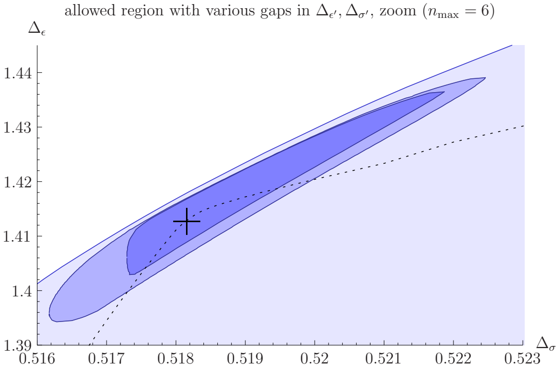
Figure 4: Zoom in on the region of the 3D Ising point in figure 3.
