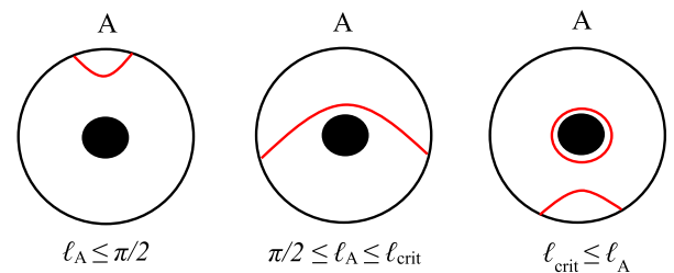
FIG. 2. The Ryu-Takayanagi surfaces for region A for the thermal ensemble \rho = \sum_i p_i \rho_i .
