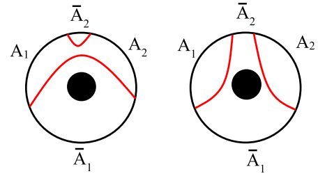
FIG. 3. Two possible Ryu-Takayanagi configurations for A_1 \cup A_2 . The total area of the surfaces on the left is S(\rho_{A_1 \cup A_2}) = S(\rho_{\bar{A}_2}) + S(\rho_{A_1 \cup \bar{A}_2 \cup A_2}) , while that on the right is S(\rho_{A_1 \cup A_2}) = S(\rho_{A_1}) + S(\rho_{A_2}) .
