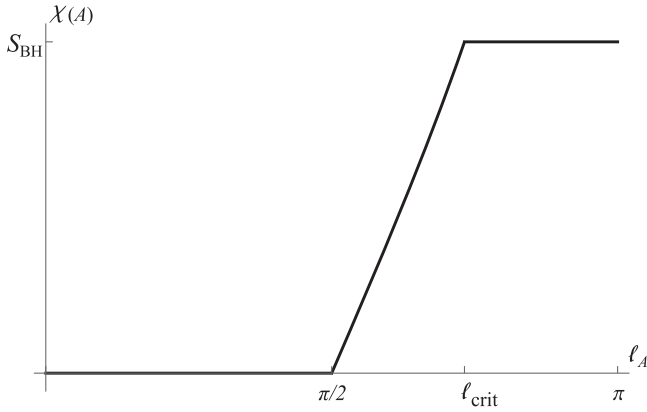
FIG. 1. The Holevo information \chi(A) in \text{AdS}_3/\text{CFT}_2 , as a function of the radius \ell_A of the subregion A . Note that \chi(A) is identically equal to zero until A covers one half of the Cauchy surface of CFT. Above this point, \chi(A) increases monotonically until it achieves the maximum value, which is the Bekenstein-Hawking entropy S_{\text{BH}} of the black hole, at \ell_{\text{crit}} defined in Sec. II.
