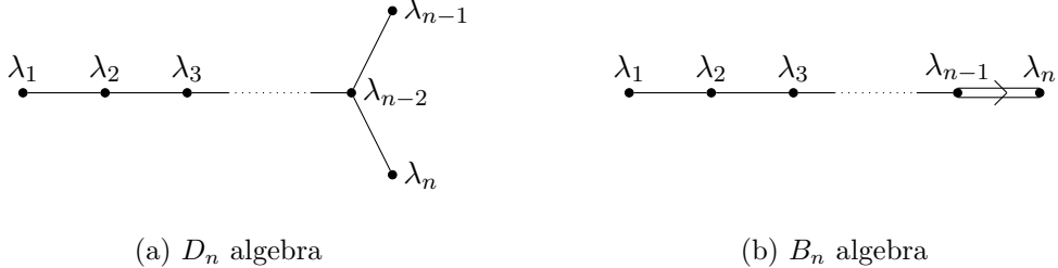
Figure 1: Dynkin diagrams of \mathfrak{so}(d) algebras.
