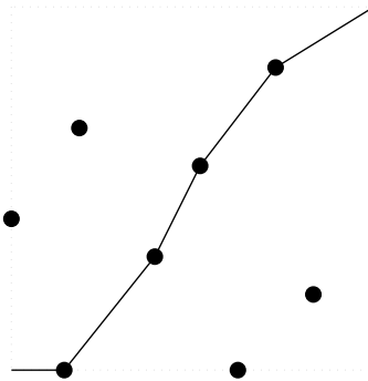
Figure 1: A points selection and the longest up/right path
