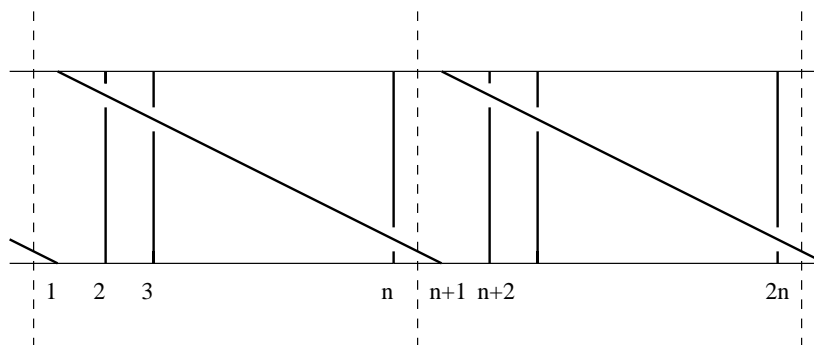
FIGURE 4. Y_1 \in B(\tilde{S}_n)
