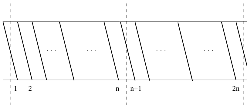
FIGURE 3. \pi \in B(\tilde{S}_n)
