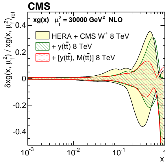
Figure 18: Relative total uncertainties of the gluon distribution at \mu_f^2 = 30\,000 \text{ GeV}^2 , shown by shaded (or hatched) bands, as obtained in the PDF fit using the DIS and W^\pm boson charge asymmetry data only, as well as single- and double-differential t\bar{t} cross sections.
