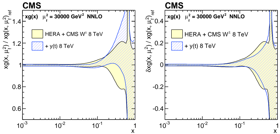
Figure 19: The gluon distribution (left) and its fractional total uncertainty (right) at \mu_f^2 = 30\,000 \text{ GeV}^2 , as obtained in the PDF fit at NNLO using the DIS and W^\pm boson charge asymmetry data only, as well as y(t) cross sections. The distributions shown in the left panel are normalized to the results from the fit using the DIS and W^\pm boson charge asymmetry data only. The total uncertainty of each distribution is shown by a shaded (or hatched) band.
