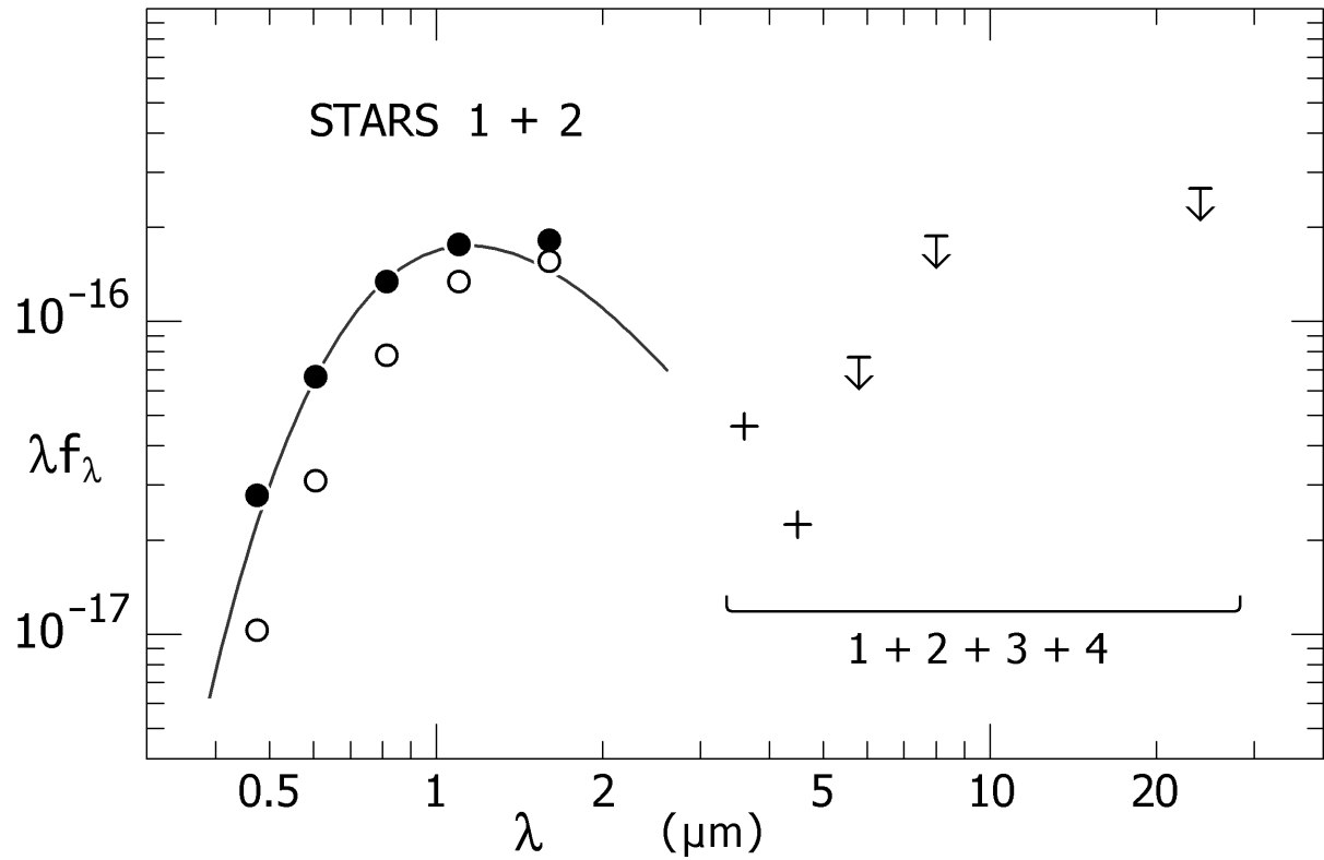
Fig. 10a.— The combined SED for the two red stars. A 3200 K Planck curve is shown for their extinction-corrected combined fluxes. Open circles are the observed fluxes based on VEGAMAGs and the filled circles are corrected for interstellar extinction, A_V = 0.8 mag. These two red stars are the probable source of near-IR flux at the position of V12. Units for \lambda f_\lambda are \text{W m}^{-2} .
