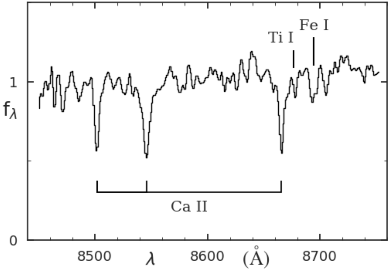
Fig. 8.— The Ca II triplet in V12. The absorption lines of Ti I( \lambda 8675 \text{\AA} ) and Fe I( \lambda 8688 \text{\AA} ) are also identified. The units are 10^{-17} ergs \text{cm}^{-2} \text{s}^{-1} \text{\AA}^{-1} .
