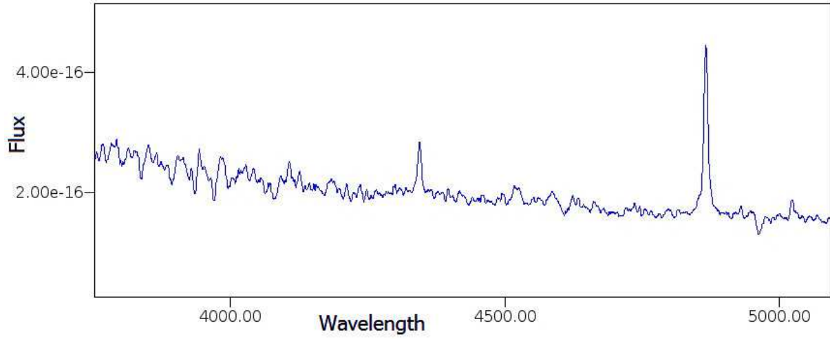
Fig. 2.— The flux calibrated ( \text{ergs cm}^{-2} \text{s}^{-1} \text{A}^{-1} ) 2003 spectrum of SN2002kg (V37).
