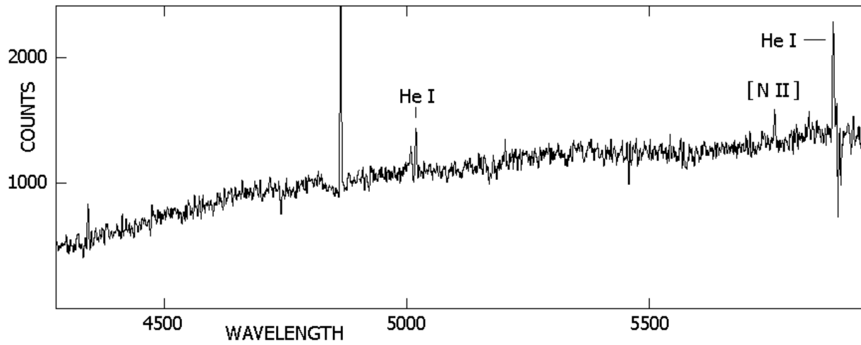
Fig. 3.— The blue spectrum of V37 from 2013. The He I \lambda 5876 lines and the [N II] line at \lambda 5755 are marked.
