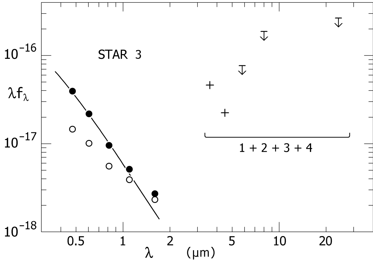
Fig. 10b.— The SED for star 3. Open circles are observed fluxes based on VEGAMAGs, and filled circles are corrected for interstellar extinction, A_V = 0.9 mag. A 25,000 K Planck curve is shown. \lambda f_\lambda is expressed in \text{W m}^{-2} .
