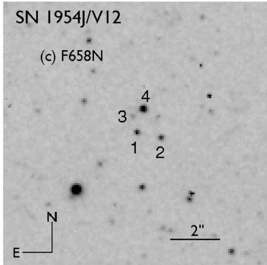
Fig. 1.— The environment of V12/SN1954j. The H \alpha HST image from Van Dyk et al. (2005b) showing the four stars.
