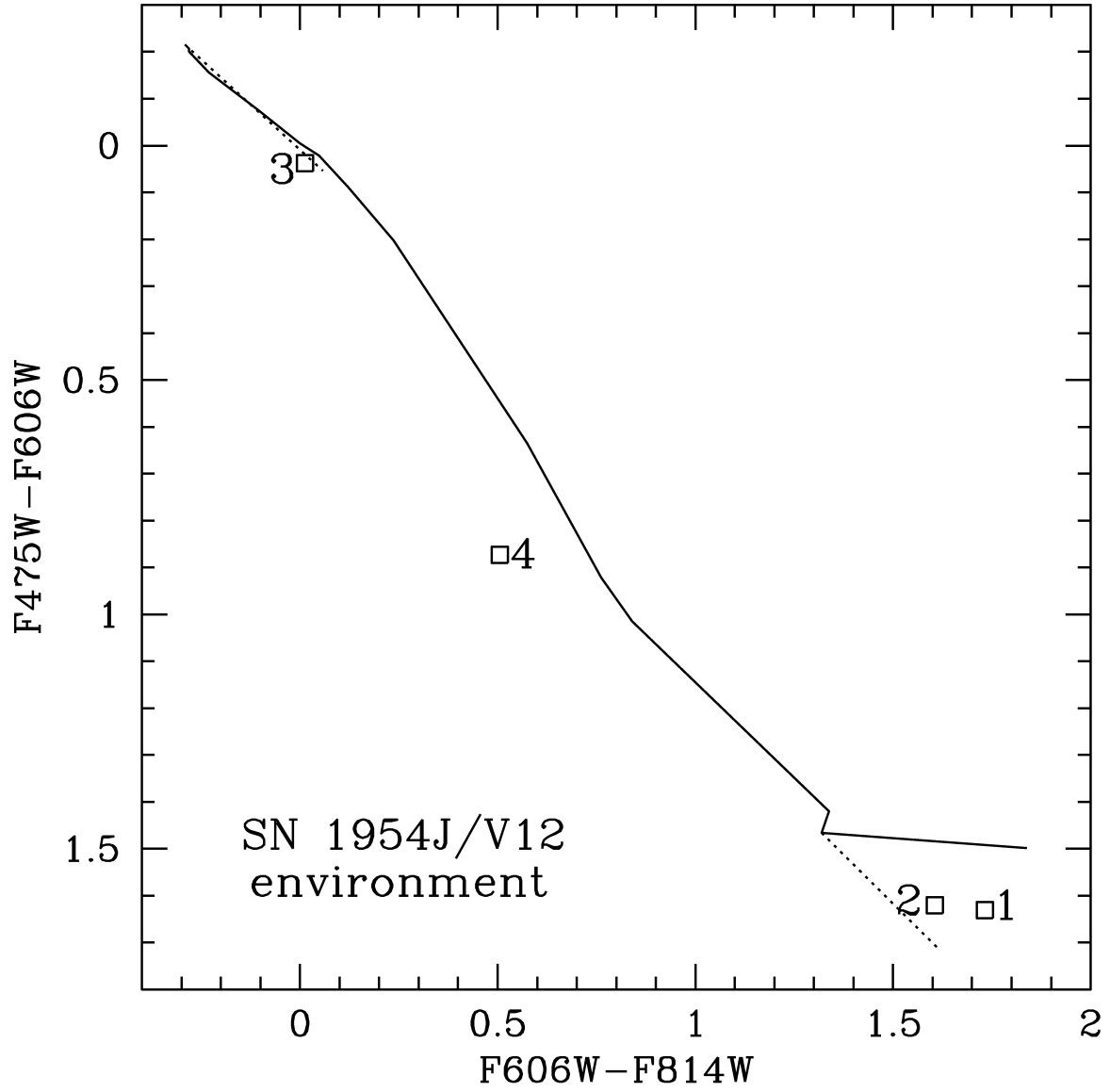
Fig. 9.— The two-color diagram for the four stars in the V12 environment using the VEGA-MAGS from 2004.
