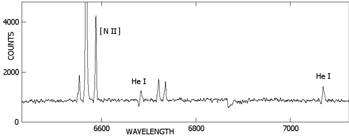
Fig. 4.— The red spectrum of V37 from 2013. The [N II] line at \lambda 6584 and two He I lines with P Cygni profiles are marked.
