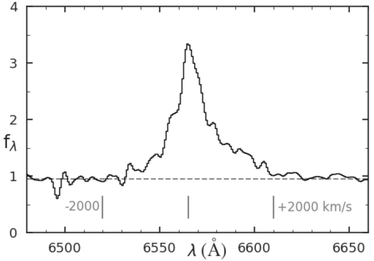
Fig. 7.— The flux calibrated H \alpha profile of V12 in 2017 January. The units for f_\lambda are 10^{-17} ergs \text{cm}^{-2} \text{s}^{-1} \text{\AA}^{-1} .
