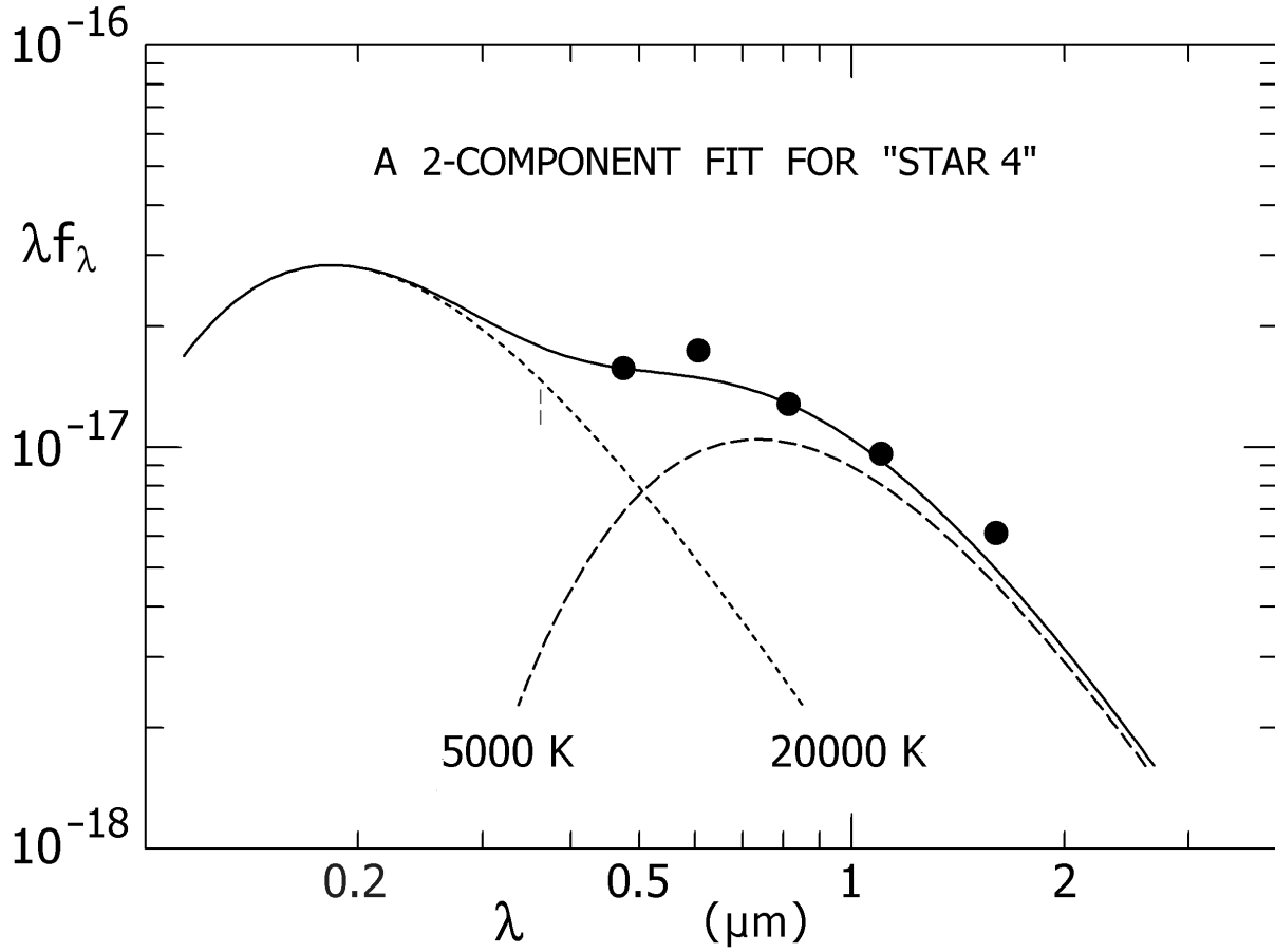
Fig. 11.— A typical two-component fit to the SED for star 4 with a 5000 K Planck curve inferred from the G-type absorption lines and a hotter 20,000 K star as discussed in Sections 4.4 and 4.6. A small vertical mark indicates the Balmer discontinuity wavelength. Possible circumstellar extinction is not included.
