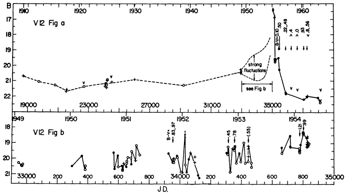
Fig. 6.— Historical light curve for V12 (SN1954J) from Tammann & Sandage (1968).
