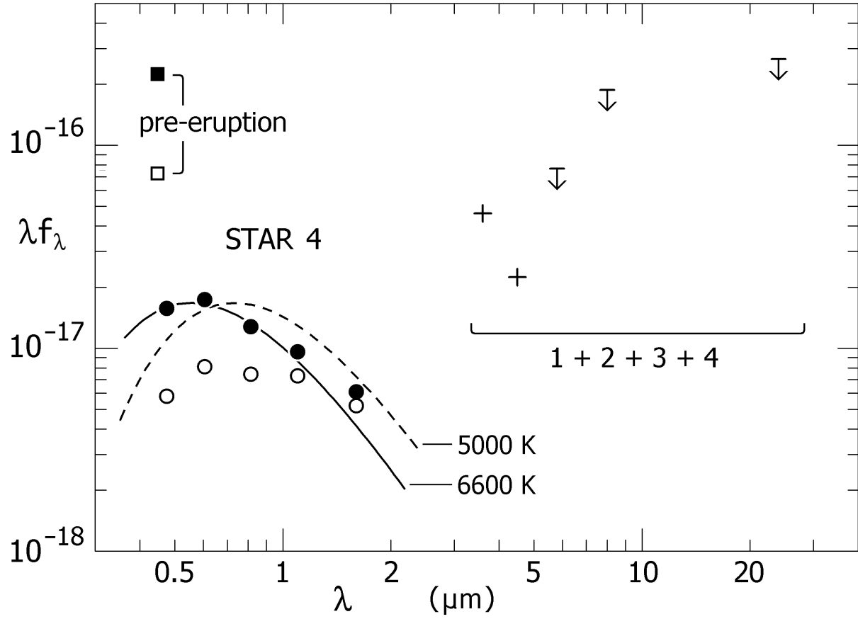
Fig. 10c.— The SED for star 4. Observed fluxes from VEGAMAGs are shown as open circles, and filled circles are corrected for interstellar extinction A_V = 0.9 mag. The best-fit Planck curve has T = 6600 K, but the absorption line spectrum indicates 5000 K. The pre-eruption magnitude in 1910–1938 is also shown. Units for \lambda f_\lambda are \text{W m}^{-2} .
