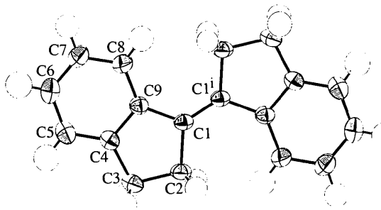
Fig. 1. An ORTEP (Johnson, 1976) drawing of the molecule with 50% probability ellipsoids. H atoms are shown as plain spheres with their refined parameters.
