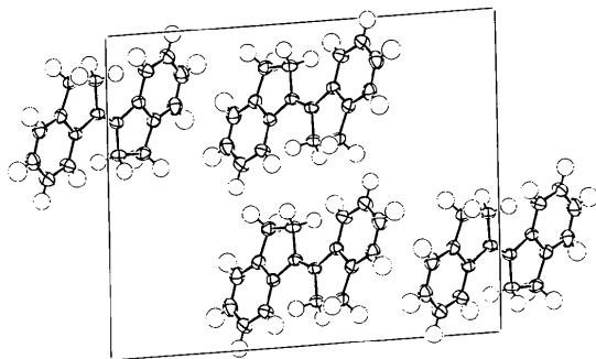
Fig. 2. An ORTEP (Johnson, 1976) drawing of the contents of a unit cell, with a unit cell outlined. Atoms are shown as in Fig. 1; the view is perpendicular to the ac plane.
