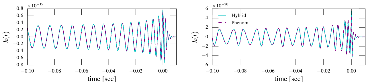
FIG. 3: Comparison between hybrid waveforms and our analytical phenomenological waveforms for a binary with total mass M = 20M_{\odot} and mass ratio q = 10 . Hybrid waveforms are constructed using all the modes with \ell \leq 4 , except the m = 0 modes. Phenomenological waveforms are constructed by taking the (discrete) inverse Fourier transform of the analytical waveforms in the Fourier domain. The left panel corresponds to a “face-on” binary (inclination angle i = 0.00 ) while the right panel corresponds to an “edge-on” binary ( i = 1.57 ).
