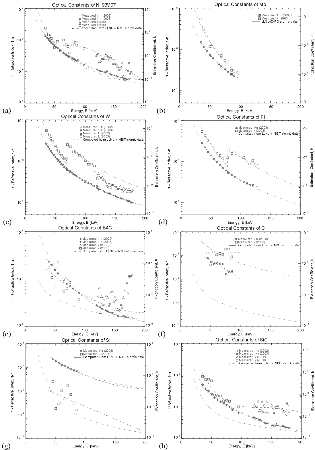
Figure 4. Optical constants ( 1-n ) and k derived from reflectance-vs-incidence angle data for (a) Ni_{.97}V_{.03} , (b) Mo , (c) W , (d) Pt , (e) B_4C , (f) C , (g) Si and (h) SiC . Measurements made in 2003 in from 35 – 120 keV are plotted as stars ( 1-n ) and squares ( k ), while measurements made in 2002 from 120 – 180 keV are plotted as crosses ( 1-n ) and triangles ( k ). The dashed lines are polynomial fits to the experimental data. The dotted lines are theoretical values computed from atomic scattering factors and mass absorption coefficients, as described in the text.
