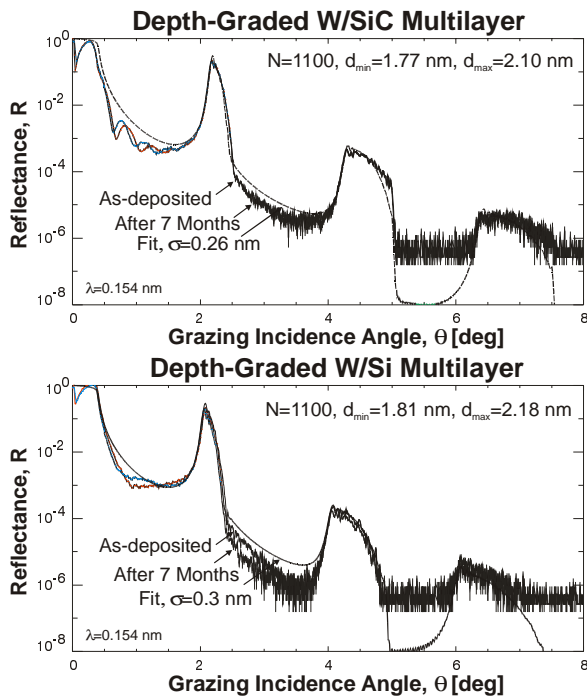
Figure 2. XRR results for depth-graded W/SiC (a) and W/Si (b) multilayers, as described in the text.
