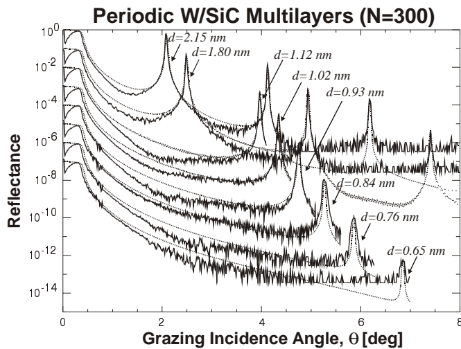
Figure 1. XRR measurements of periodic W/SiC multilayers containing N=300 bilayers, with periods d as indicated. For clarity, each curve is offset by a factor of 10 from the previous curve. Fits to the measured data are shown as dotted lines.
