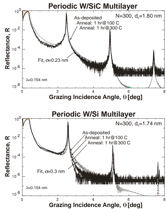
Figure 3. XRR results for periodic W/SiC (a) and W/Si (b) multilayers comparing the as-deposited films with those annealed for 1 hr at 100 C and 300 C, as indicated.
