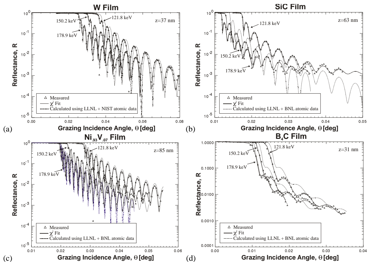
Figure 5. X-ray reflectance-vs-graze angle curves for single-layer films of (a) W, (b) SiC, (c) Ni 93 V 07 , and (d) B 4 C. The film thicknesses, determined from XRR, are indicated in each case. Curves obtained at E=121.8 keV, 150.2 keV, and 178.9 keV are indicated. \chi^2 minimization fits to the measured data are shown as solid lines. The dotted lines are the reflectance curves calculated using optical constants computed from theoretical atomic scattering factors and mass absorption coefficients that account for incoherent scattering.
