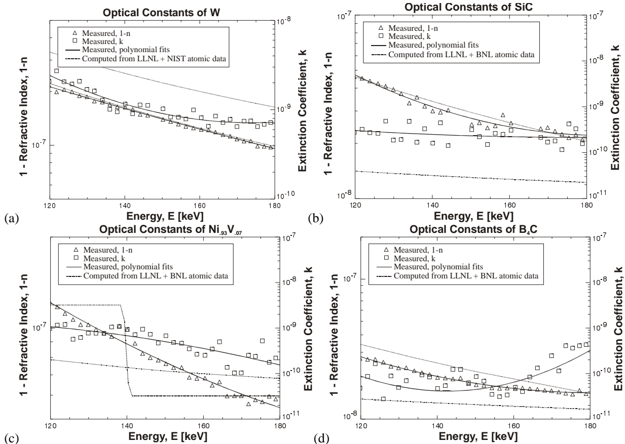
Figure 6. Optical constants ( 1-n ) [triangles] and k [squares] derived from reflectance-vs-incidence angle data for (a) W, (b) SiC, (c) Ni 93 V 07 , and (d) B 4 C. The solid lines are polynomial fits to the experimental data. The dotted lines are theoretical values computed from atomic scattering factors and mass absorption coefficients, as described in the text.
