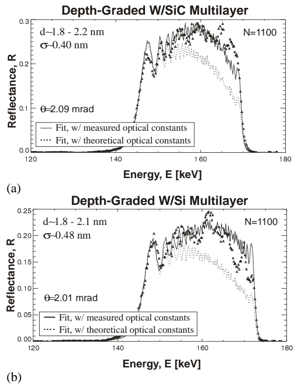
Figure 4. Hard X-ray reflectance of depth-graded W/SiC (a) and W/Si (b) multilayers measured using synchrotron radiation. The solid lines are calculations made using experimentally-determined optical constants, while the dotted lines are calculations made using theoretical optical constants, as described in §5.
