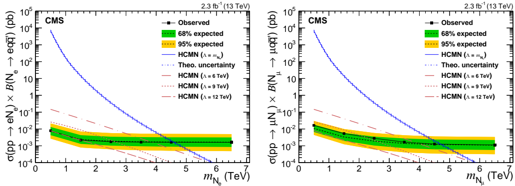
Figure 5: The observed 95% CL upper limits (solid black lines) on \sigma(\text{pp} \rightarrow \ell N_\ell) \mathcal{B}(N_\ell \rightarrow \ell \bar{q}\bar{q}') , obtained in the analysis of the ee\bar{q}\bar{q}' (left) and the \mu\mu\bar{q}\bar{q}' (right) final states, as a function of the mass of the heavy composite Majorana neutrino, N_\ell . The corresponding expected limits are shown by the dotted lines, and the bands represent the expected variation of the limit to one and two standard deviation(s). The solid blue curve indicates the theoretical prediction of \sigma(\text{pp} \rightarrow \ell N_\ell) \mathcal{B}(N_\ell \rightarrow \ell \bar{q}\bar{q}') for \Lambda = m_{N_\ell} . The uncertainty in the theoretical prediction is derived by taking into account the factorization and normalization scales. The light red textured curves give the theoretical predictions for three \Lambda values ranging from 6 to 12 TeV in steps of 3 TeV.
