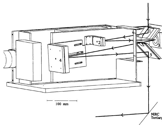
FIG. 1—Diagram of the Image Magnifier (IM) in its deployed position. A central ray is traced through the five mirrors, which are numbered according to their order, as described in the text. The light enters from the top of the drawing, and exits at the bottom. The fold mirror, shown at the bottom right, is mounted onto NIRC and is the tertiary mirror under direct-imaging conditions; when the IM stage is deployed, it instead takes light from the IM into NIRC.
