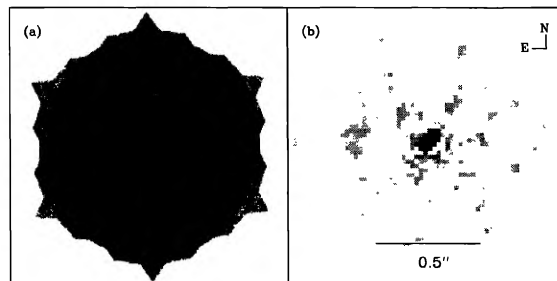
FIG. 4—(a) The power spectrum ( |O(\mathbf{u})|^2 from Eq. 1) of the binary star \beta LMi (SAO 62053), which has a somewhat mottled appearance due to small miscalibrations of the individual segments. With only 100 exposures, this effect limited the dynamic range to 3.5 mag. (b) The final diffraction-limited image of \beta LMi showing the binary with a separation of 0''.06 and flux ratio of 2.4 mag.
