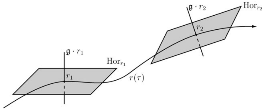
Figure 2. Geometry of the method of connections.
