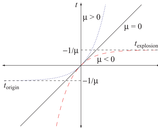
Figure 3. Qualitative behaviour of scaling laws. For \mu > 0 , the self-similar solution exists for all positive time, and t = -1/\mu is the ‘virtual origin.’ For \mu < 0 there is a finite-time singularity (either explosion or implosion) at t = -1/\mu > 0 . In the scaled time \tau , self-similar solutions exist for all time, regardless of the value of \mu .
