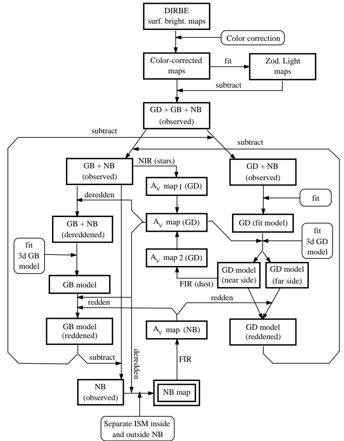
Fig. 3. Flow chart of the COBE data reduction steps
