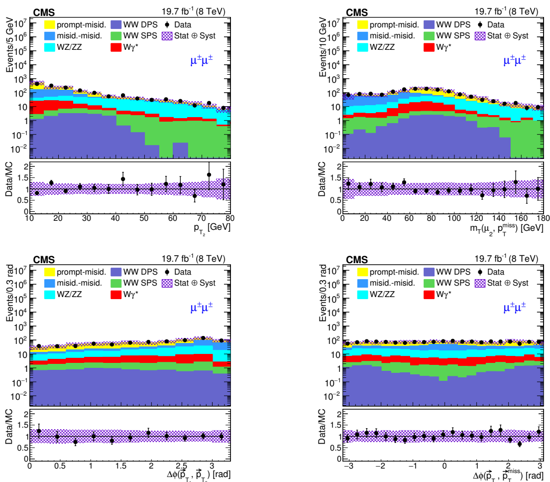
Figure 2. Distributions of the p_{T_2} (top-left), m_T(\mu_2, p_T^{\text{miss}}) (top-right), \Delta\phi(\vec{p}_{T_1}, \vec{p}_{T_2}) (bottom-left), and \Delta\phi(\vec{p}_{T_1}, \vec{p}_T^{\text{miss}}) (bottom-right) variables for the dimuon channel, after the same-sign WW selection criteria have been applied. The data are represented by the black dots and the shaded histograms represent the predicted signal and background processes normalized according to the estimated cross sections and the luminosity. For each individual distribution, the bottom panels show the ratio of the number of events observed in the data to that predicted by the simulation, along with the associated statistical uncertainty. The hatched bands in all cases represent the sum of the systematic and statistical uncertainties of the simulated samples, added in quadrature.
