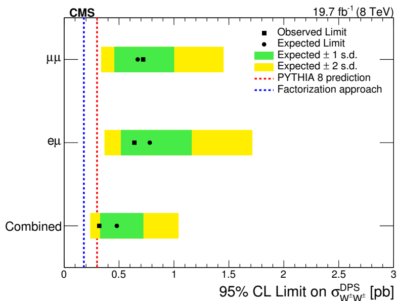
Figure 5. Expected and observed 95% CL upper limits on the same-sign \sigma_{W^\pm W^\pm}^{\text{DPS}} for the dimuon and electron-muon final states, along with their combination. The predicted values of \sigma_{W^\pm W^\pm}^{\text{DPS}} from PYTHIA8 and from the factorization approach [21] are also shown.
