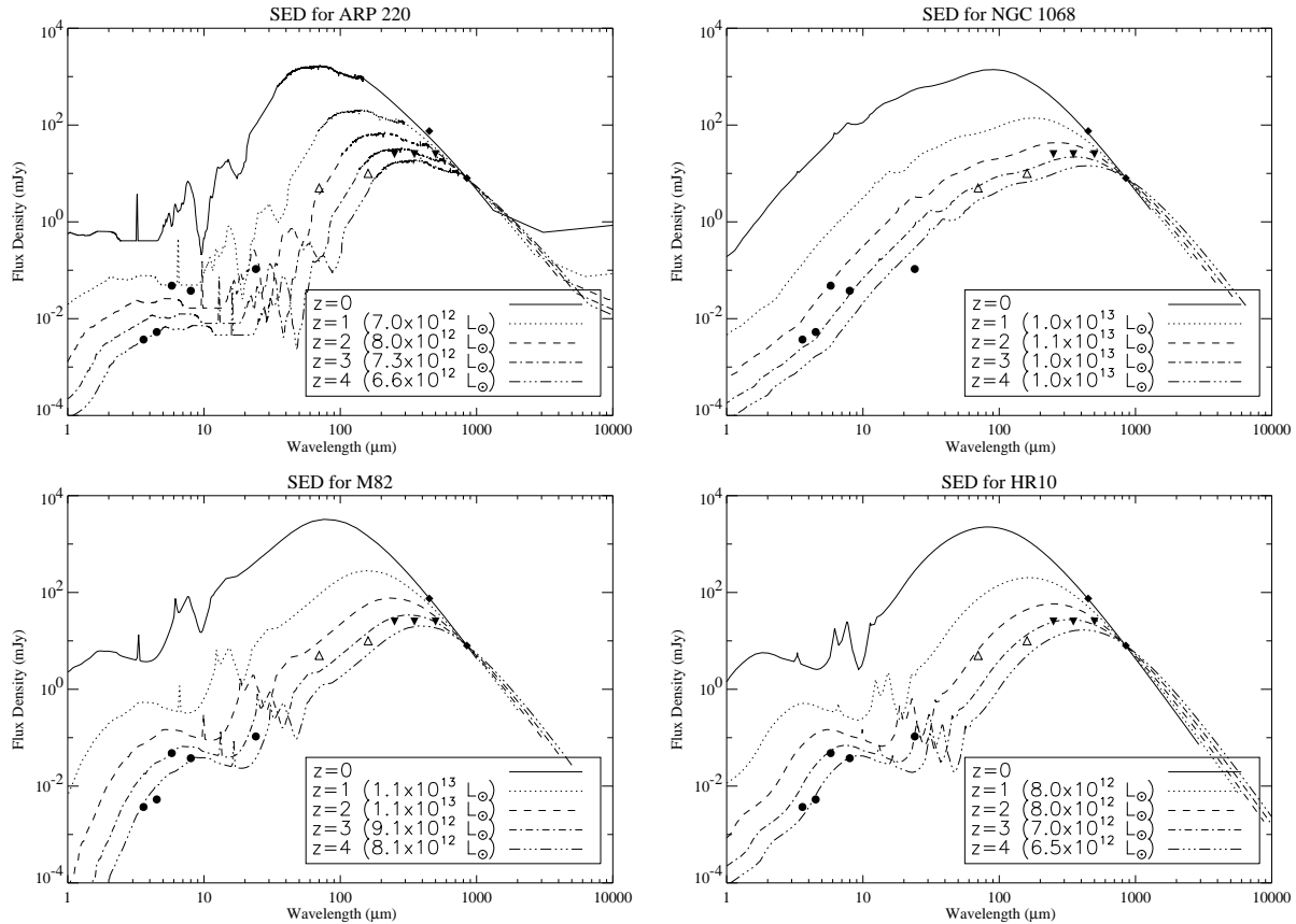
Figure 1. Model spectral energy distribution plots of template galaxies with survey sensitivities overplotted. Filled circles: SWIRE sensitivities 500 seconds, 5\sigma (Lonsdale et al. 2004). Open triangles: The pre-flight Spitzer sensitivities for 70 and 160 \mu\text{m} are shown whilst the SWIRE team re-assess their observing strategy due to the degraded MIPs sensitivities, although currently these are expected to be two to three times worse. Filled triangles: The pre-flight BLAST confusion limit estimates (derived from Rowan-Robinson 2001) of 25 mJy; the sensitivity estimates (Hughes et al. 2002) are in the range 15 – 25 mJy. Filled diamonds: SHADES survey sensitivities of 8 mJy at 850 \mu\text{m} and 75 mJy at 450 \mu\text{m} . Models have been normalised to the SHADES survey depth of 8 mJy at 850 \mu\text{m} . Top left panel: Arp 220 – a highly-obscured local starburst galaxy (note: it is also a ULIRG Elbaz et al. 2002). Top right panel: NGC1068 – a typical Seyfert galaxy (Efsthathiou, Hough & Young 1995). Bottom left panel: M82 – an irregular dusty star-forming galaxy (Efsthathiou, Rowan-Robinson & Siebenmorgen 2000). Bottom right panel: HR10 – a high-redshift, extremely-red galaxy (Takagi, Hanami & Arimoto 2004). Bolometric (3–1000 \mu\text{m} rest-frame) luminosities for each model, as normalised, are shown in the legends.
