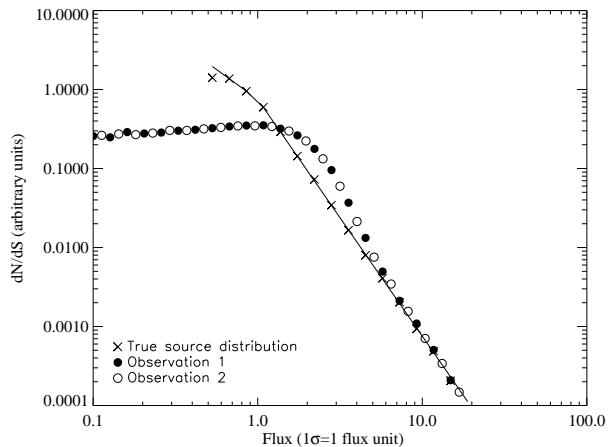
Figure 10. A simulation of Eddington bias for a sample of 10,000 sources with one \sigma equal to one flux unit. Although flux boosting does occur for a fraction of the simulated sources, the actual sources detected between 3\text{--}3.5\sigma varies between individual observations because of the random effect of the noise. Of the 10,000 sources simulated here, \sim 2600 were found with S/N between 3\text{--}3.5\sigma in the first and/or second observations, but only 535 were found with S/N in the range 3\text{--}3.5\sigma in the first observation and > 3\sigma in the second. Therefore, when applying a significance threshold, the lower-significance source lists derived from each observation are markedly different, despite the fact that both observations yield clearly consistent Eddington-biased source counts.
