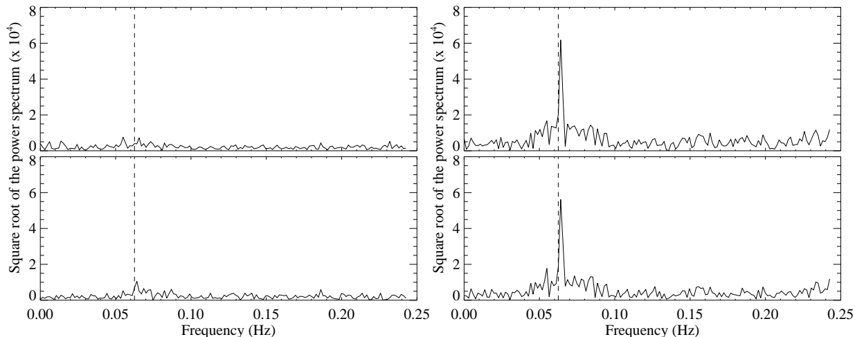
Figure 3. The spike in the power spectrum of the bolometer readouts. The upper row of plots shows the power spectrum of a typical (in this case the central) bolometer, before (left) and after (right) sky subtraction. The lower row of plots shows the same for a bolometer affected by the power-spike, showing clearly the spike at a period of roughly 16 samples (at the dotted line) and the fact that the power-spike itself has not changed.
