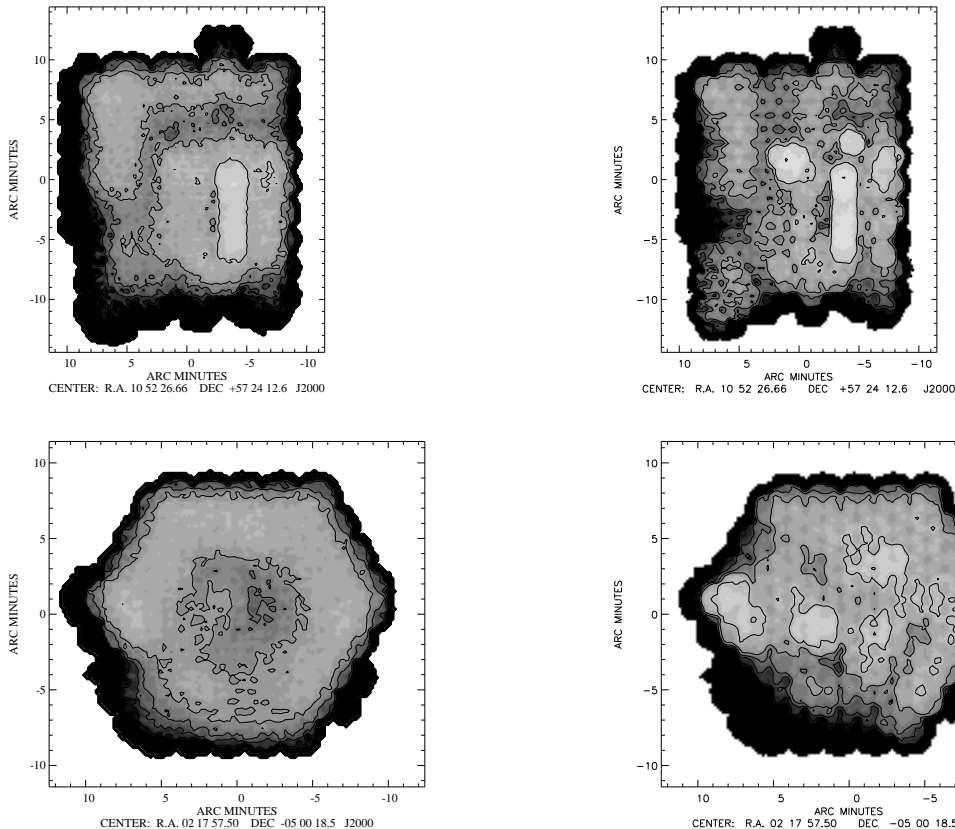
Figure 7. Noise maps of the ( Top Row ) Lockman Hole East and ( Bottom Row ) SXDF for data taken up to February 2004. For the 850\ \mu\text{m} data ( Left Column ), the lowest contour level is 0.71\ \text{mJy} with higher contours spaced by 0.71\ \text{mJy} to a maximum level shown in the map of 5\ \text{mJy} . For the 450\ \mu\text{m} data ( Right Column ), the lowest contour level is 7.1\ \text{mJy} with higher contours spaced by 7.1\ \text{mJy} to a maximum level in the map of 50\ \text{mJy} . Note the high levels of noise around the edges of the map, which will be reduced when more observations are taken.
