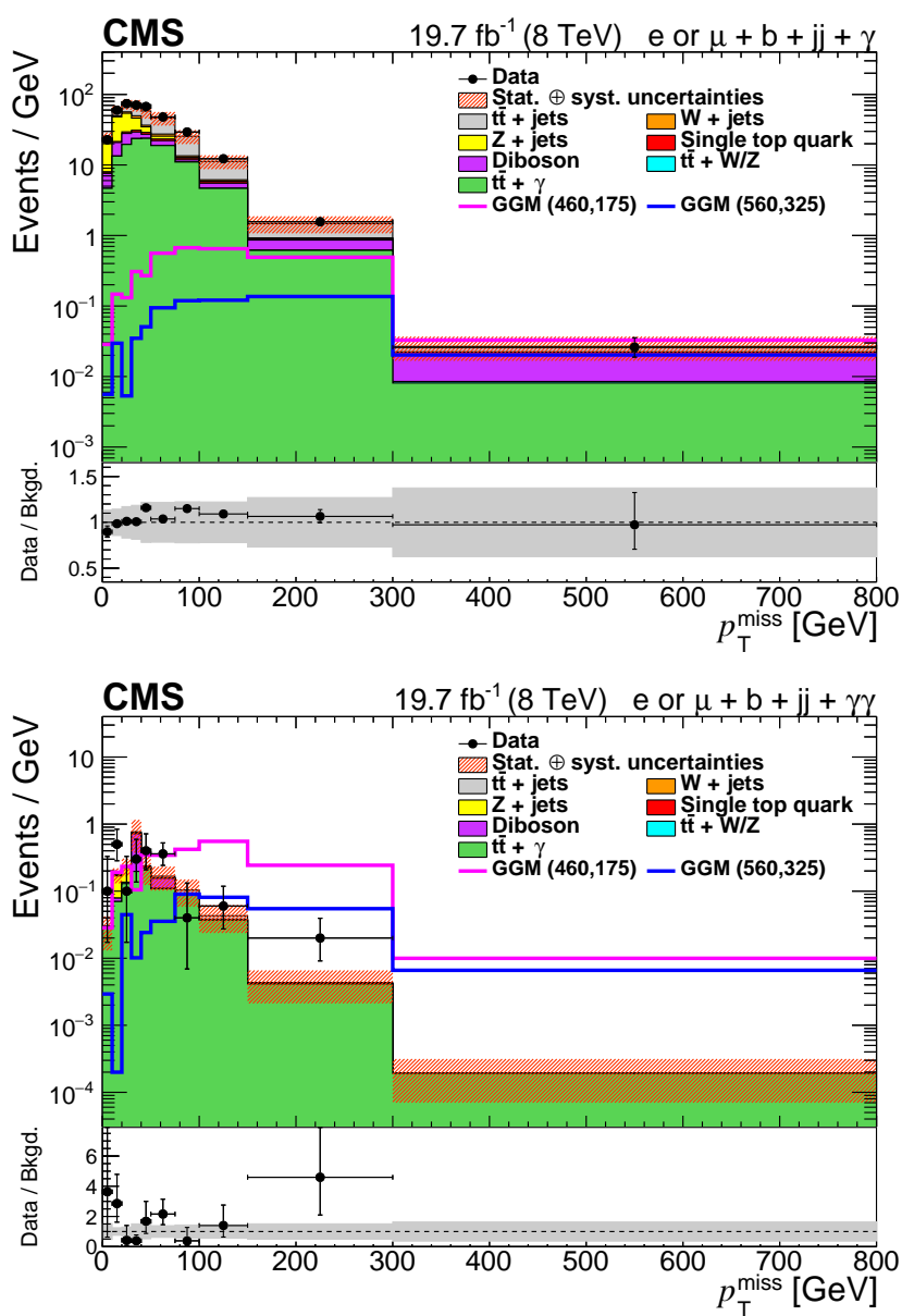
Figure 4: Comparison of data and MC simulation in p_T^{\text{miss}} for the combined (e and \mu ) signal regions: (upper pane) SR1 with one reconstructed photon and (lower pane) SR2 with two reconstructed photons. Each bin is normalized by its bin width.
