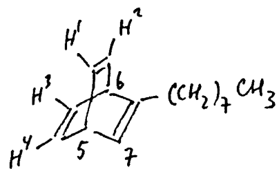
Compd. 196
