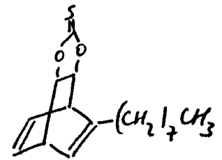
compd. 186
