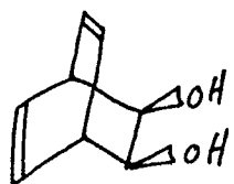
Compd. 17a
