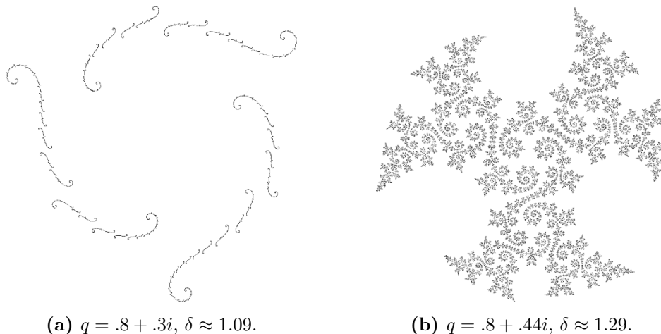
Figure 2. The limit sets for two of the \mathbb{Z}_3 symmetric genus two Schottky groups that arise when investigating n = 3 Rényi entropies. The parameter q defining the groups is an eigenvalue of one of the generators as specified in section 2.3. We give the value of the Hausdorff dimension \delta for these two limit sets, computed using the methods of section 5.
