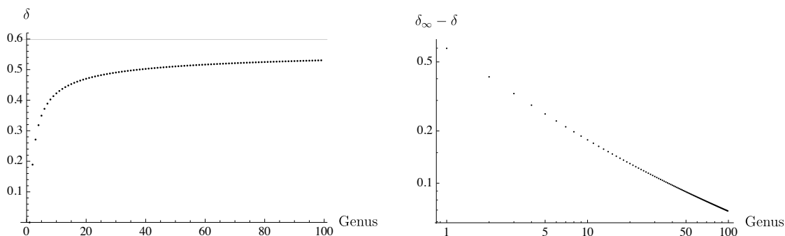
Figure 5. The critical dimension for the x = \frac{1}{2} Rényi surface as a function of replica number n . The asymptote is the computed limit as n \rightarrow \infty . On the right is a log-log plot showing convergence to this value.
