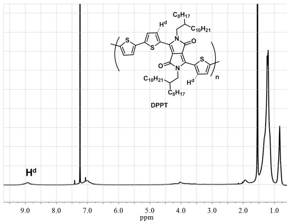
Figure S2. DPPT ^1\text{H} spectrum.
