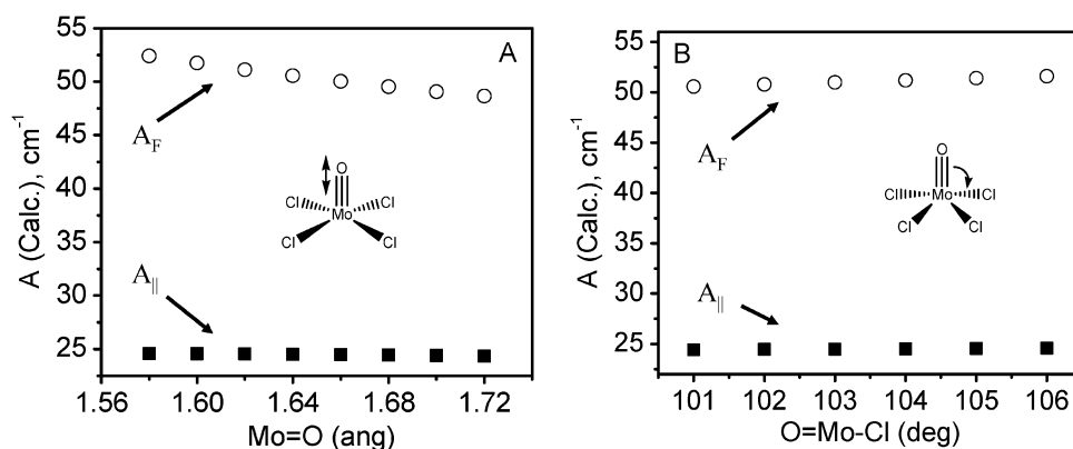
Fig. 3 Graphical representation of the dependence of the calculated A_F term (circles) and A_{\parallel} (squares) values on the (A) Mo=O bond distance and (B) O=Mo-Cl angle for [\text{MoOCl}_4]^- using a B3P86 XC functional and a RESC scalar relativistic correction.
