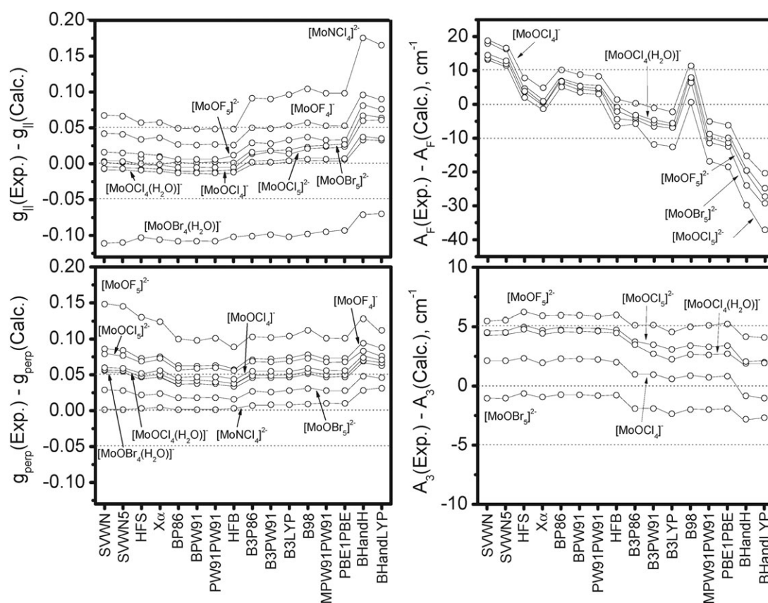
Fig. 4 Differences between experimental and calculated g_{\parallel} (experimental data available for 8 complexes), g_{\perp} (experimental data available for 8 complexes), A_F (experimental data available for 5 complexes), and A_3 (the largest anisotropic component) (experimental data available for 5 complexes) EPR parameters for molybdenum(v) compounds, using BP86 optimized geometries and BS1. The complexes with the largest deviations are labeled.
