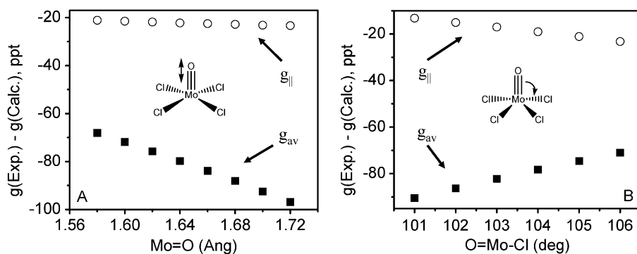
Fig. 2 Graphical representation of the dependence of the calculated g_{\parallel} (circles) and average ( g_{\text{av}} ) values (squares) [where g_{\text{av}} = 1/3(g_x + g_y + g_z) ] on (A) the Mo=O bond distance and (B) the O=Mo-Cl bond angle for [\text{MoOCl}_4]^- using a B3P86 XC functional and a RESC scalar relativistic correction.
