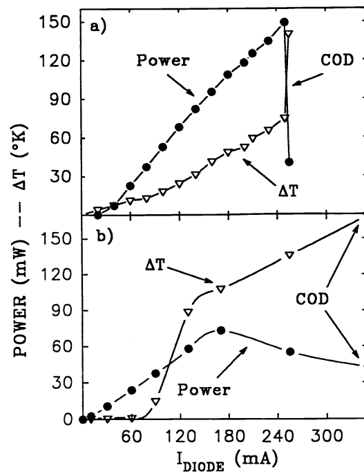
Figure.2. Output power and cladding layer temperature shift as a function of diode current I_d for coated AlGaAs-based with non deoxidized facets (a) and uncoated InGaP-based (b) diode lasers.
