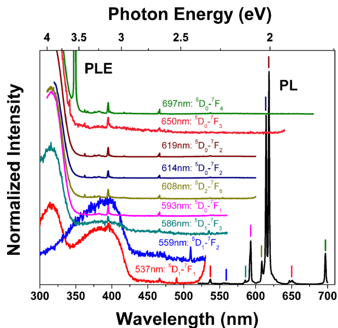
FIG. 3. PL and PLE spectra for as-grown \text{YVO}_4:\text{Eu}^{3+} . PL data were captured for an excited wavelength of 250\text{ nm} and PLE data were monitored at each of the labeled transitions. PLE spectra are vertically offset for clarity.
