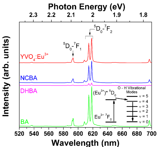
FIG. 4. Emission spectra of as-grown and treated \text{YVO}_4:\text{Eu}^{3+} nanoparticles excited at 250 nm. The attached aromatic molecules are BA, NCBA, and DHBA. Spectra are vertically offset for clarity. The inset shows a schematic diagram of alignment of \text{Eu}^{3+} energy gap with O-H vibrational modes.
