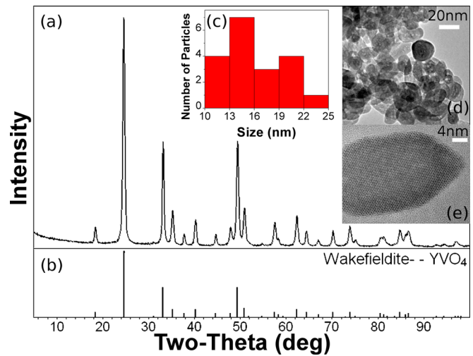
FIG. 1. (a) X-ray diffraction pattern from the as-grown \text{YVO}_4:\text{Eu}^{3+} nanoparticles with (b) the expected peak structure given in the International Center for Diffraction Database. Nanoparticle size dispersion histogram (c) measured from diameters. Transmission electron micrographs of samples with (d) 20 nm and (e) 4 nm scale bars.
