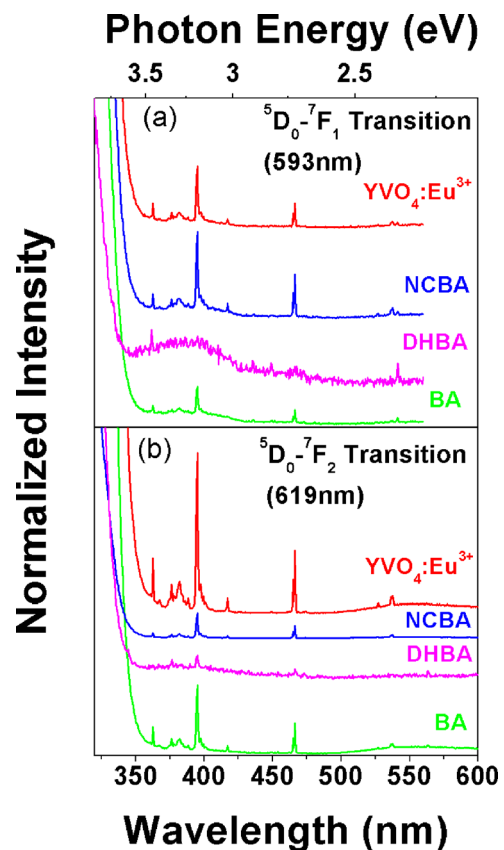
FIG. 5. Photoluminescence excitation spectra for as-grown and treated \text{YVO}_4:\text{Eu}^{3+} nanoparticles for the (a) magnetic-dipole {}^5\text{D}_0\text{-}{}^7\text{F}_1 transition at 593 nm and (b) electric-dipole {}^5\text{D}_0\text{-}{}^7\text{F}_2 transition at 619 nm. Spectra are normalized to the peak emission at the respective wavelengths and offset for clarity.
