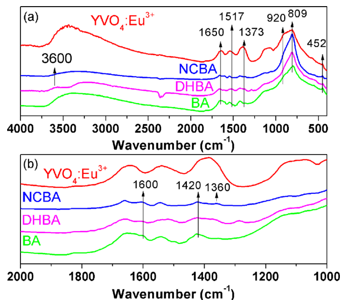
FIG. 2. Fourier transform infrared spectra of \text{YVO}_4:\text{Eu}^{3+} nanoparticles and \text{YVO}_4:\text{Eu}^{3+} with attached aromatic linker molecules BA, NCBA, and DHBA for the wavelength ranges (a) 4000\text{--}400 \text{ cm}^{-1} and (b) 2000\text{--}1000 \text{ cm}^{-1} . Spectra are vertically offset for clarity.
