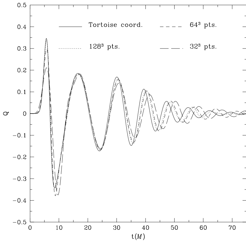
FIG. 4. Same as Figure 3 for \ell = 4 .
