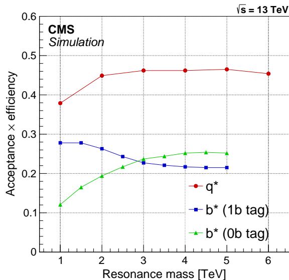
Figure 1: The product of acceptance and efficiency for q^* and b^* signals as a function of generated m_{q^*} or m_{b^*} mass, calculated using MC simulation.
