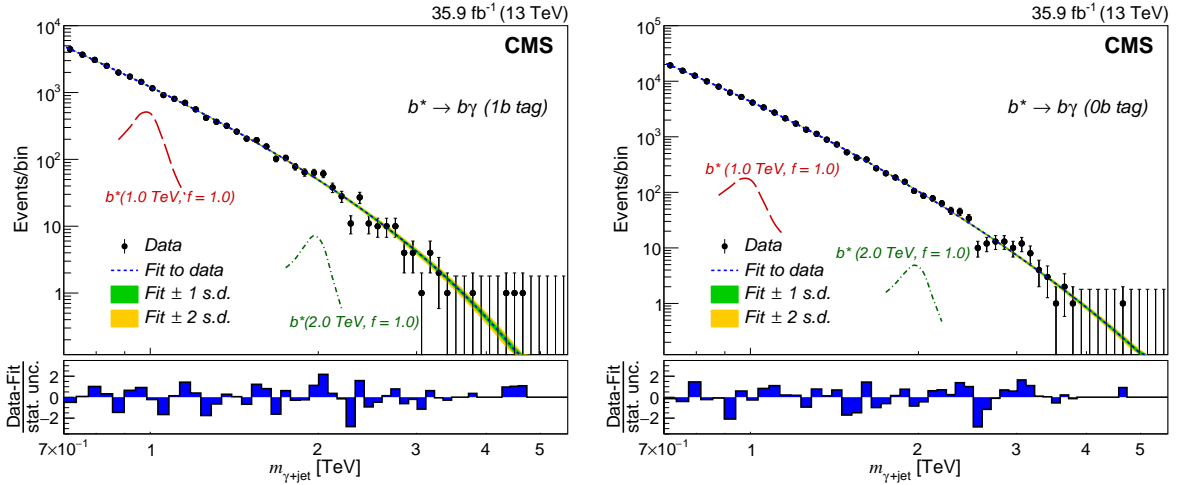
Figure 3: The \gamma +b jet invariant mass distribution in data (black points) used for the b^* analysis, after final selection for (left) 1b tag category and (right) 0b tag category. The result of the fit to the data using the parametrization defined in Eq. (2) is shown by the blue dashed curve with associated bands indicating the uncertainty. The bin-by-bin pull, (\text{Data-Fit})/(\text{stat. unc.}) , where the denominator refers to the statistical uncertainty in data, is also presented. The green and yellow bands correspond to 1 and 2 standard deviations, respectively from the mean value. Simulations of excited b quark signals representing the expected excess of signal events over the background are shown for the 1b and 0b tag categories for the mass values of 1.0 and 2.0 TeV for f = 1.0 .
