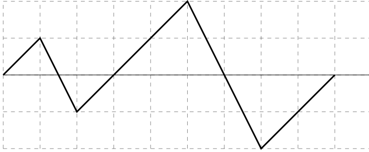
Figure 4. An example of a bridge (an unconstrained analog of an excursion) made of the same elementary steps as the excursion in fig. 3.
