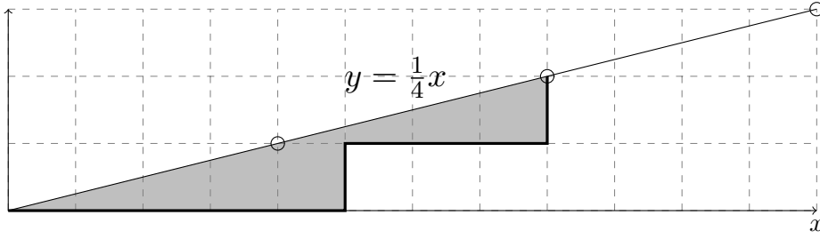
Figure 2. A lattice path under the line y = \frac{1}{4}x , and a shaded area between the path and the line.
