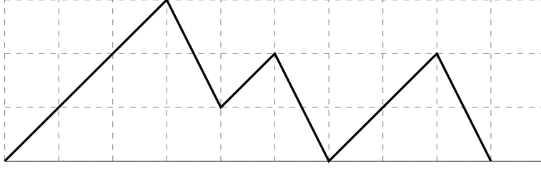
Figure 3. Counting of paths under the line y = \frac{1}{2}x is equivalent to counting excursions , i.e. paths in the upper half plane, made of elementary steps (1, 1) and (1, -2) .
