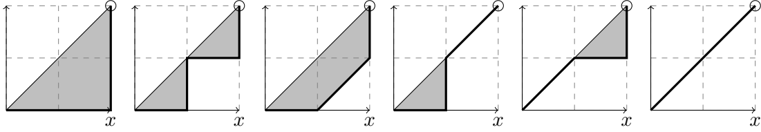
Figure 7. All 6 Schröder paths represented by quadratic terms (q^2 + q^4)x_1^2 + (2q + q^3)x_1x_2 + x_2^2 of the generating function (6.6).
