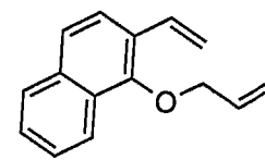
Compound 2j/ \text{CD}_2\text{Cl}_2
