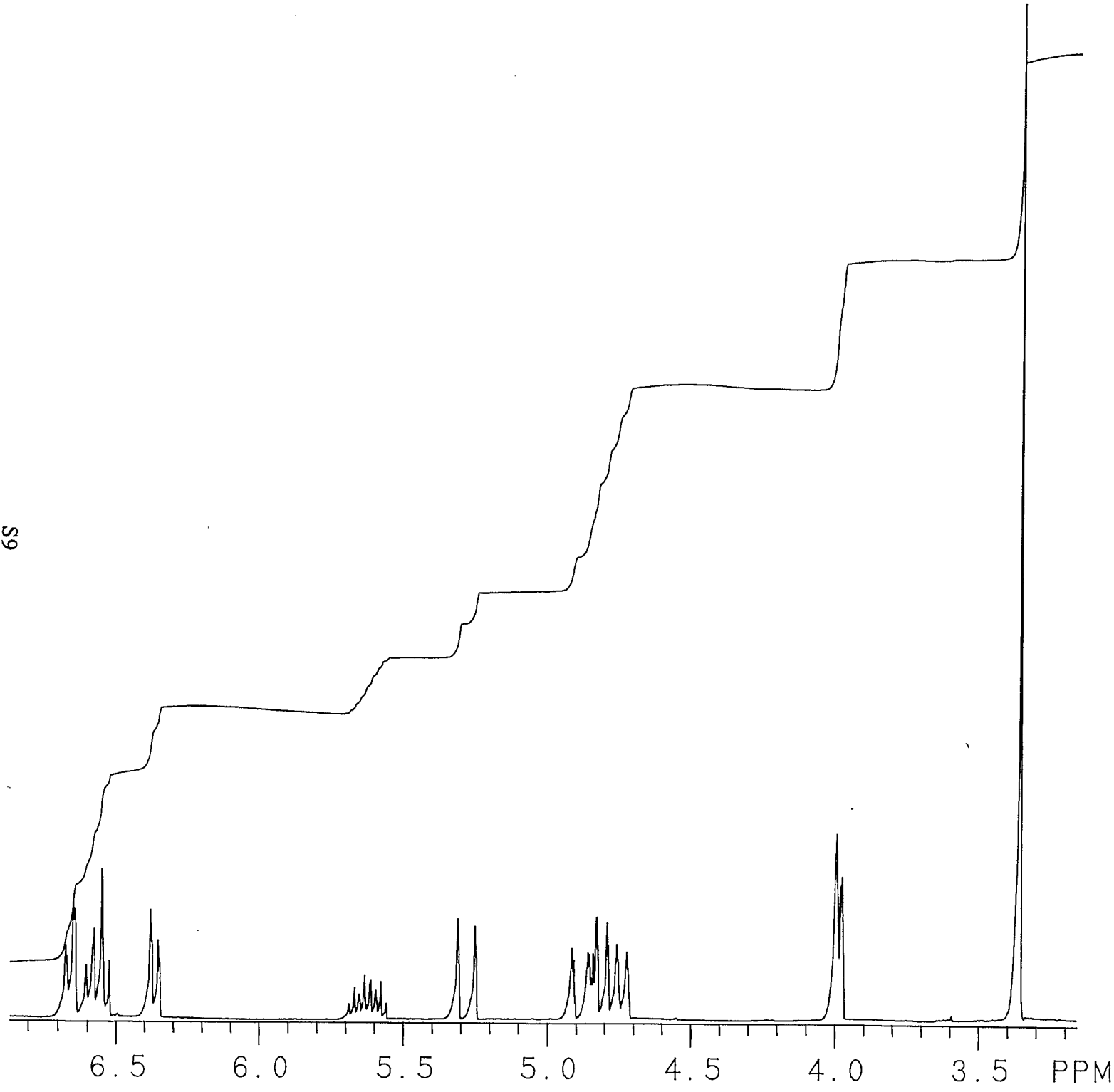
Compound 2h/CD 2 Cl 2
