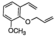
Compound 2h/CD 2 Cl 2
