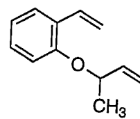
Compound 2k /CD 2 Cl 2
