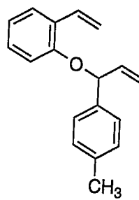
Compound 2 /CD 2 Cl 2
