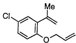
Compound 2f /CD 2 Cl 2
