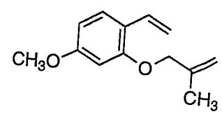
Compound 2g/CD 2 Cl 2
