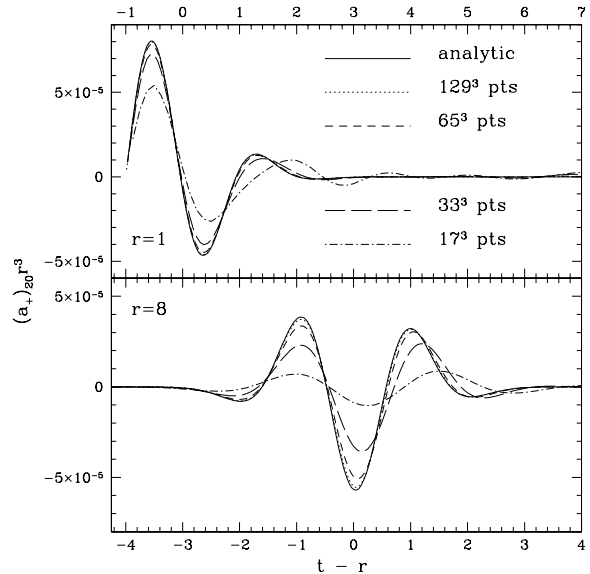
FIG. 2. Convergence to the analytic solution of the extracted ( r = 1 ) and evolved ( r = 8 ) multipole (a_+)_{20} . The amplitude is scaled by r^3 to compensate for the radial fall-off.
