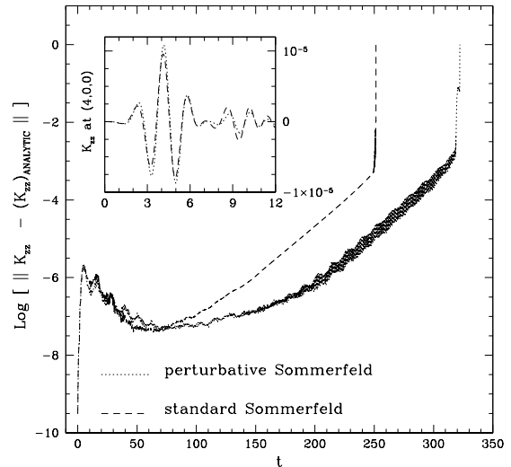
FIG. 4. Long-term evolution of the L_2 norm of the error in K_{zz} at the 3D outer boundary surface. The inset shows K_{zz} at the outer boundary along the x -axis. The interior grid has (33)^3 gridpoints and the code is stopped when the norm is unity.
