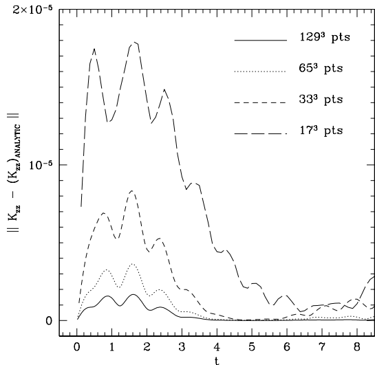
FIG. 3. Convergence to zero of the L_2 norm of the error of K_{zz} integrated over the 3D outer boundary surface.
