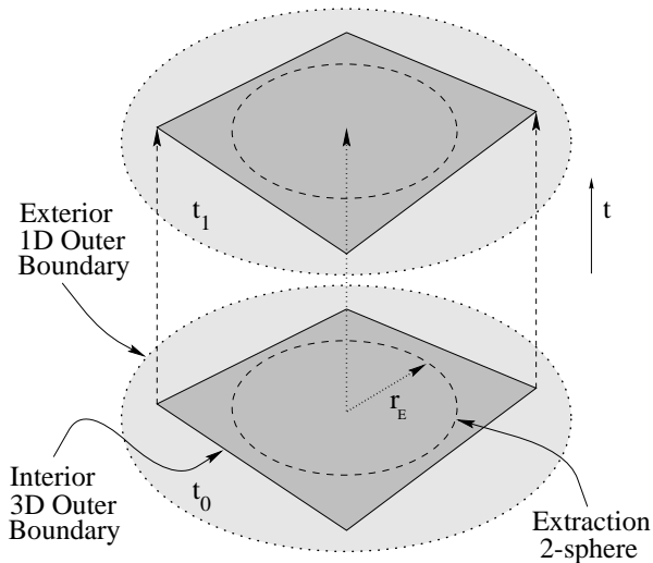
FIG. 1. Location of the different outer boundaries and of the extraction 2-sphere for two successive timeslices. The dark shaded region shows the spatial domain over which the 3D nonlinear equation are solved.
