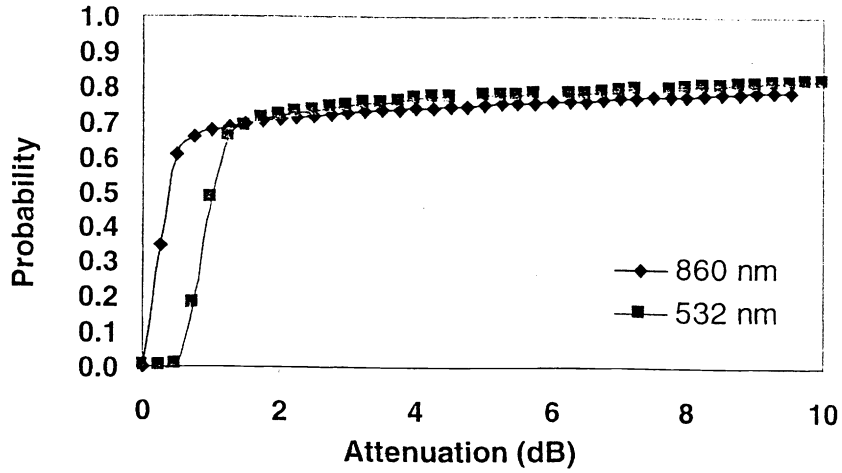
Figure 3. Attenuation CDF for Mt. Lemmon during November 1996 at 532 and 860 nm.
