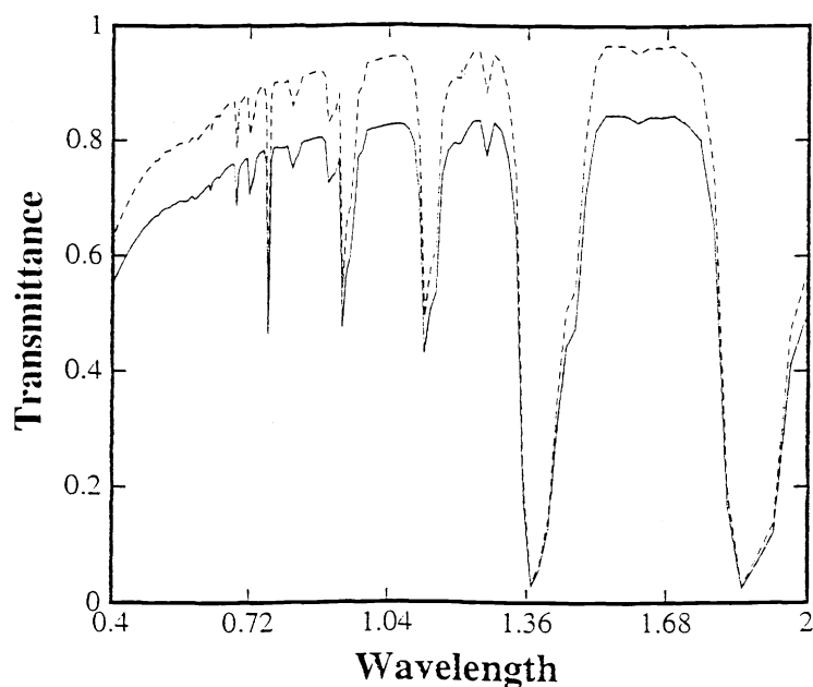
Figure 5. Atmospheric transmission at zenith as a function of wavelength for a 2 km altitude site generated from MODTRAN [6]. The two curves are for clear sky and high cirrus clouds. Note: both TMF and Mt. Lemmon are at altitudes slightly higher than 2 km.
