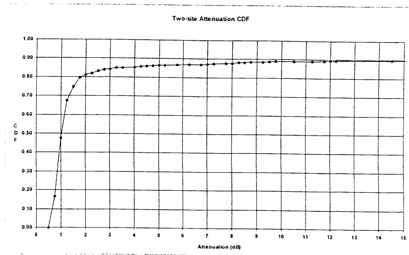
Figure 6. Two-site joint CDF for Mt. Lemmon and TMF during November 1996 at 532 nm.
