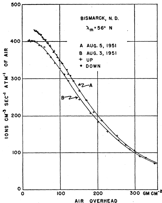
FIG. 4. Representative curves for two particular days at Bismarck, geomagnetic latitude, \lambda_m , 56°N.
