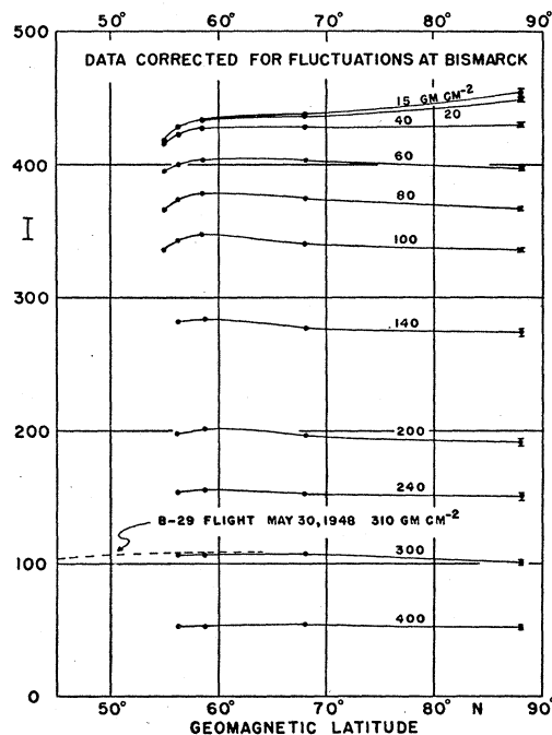
FIG. 14. After corrections are made to the flights at intermediate latitudes and at Thule, the data show much more consistency than is evident in Fig. 13. The uncertainties indicated at 88^{\circ}\text{N} are the resultant extremes of the 4 simultaneous flights after corrections are made.
