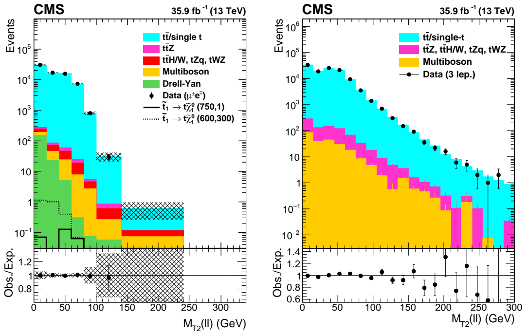
Figure 3: Left: distribution of M_{T2}(\ell\ell) in a control region enriched in t\bar{t} events and defined by N_{\text{jets}} \geq 2 , N_{b\text{jets}} \geq 1 , and p_T^{\text{miss}} < 80 \text{ GeV} . The hatched band shows the uncertainties from experimental effects, as described in Section 7. Right: distribution of M_{T2}(\ell\ell) after swapping an isolated lepton with an additional non-isolated lepton, as described in the text. For both plots, simulated yields are normalized to data using the yields in the M_{T2}(\ell\ell) < 100 \text{ GeV} region.
