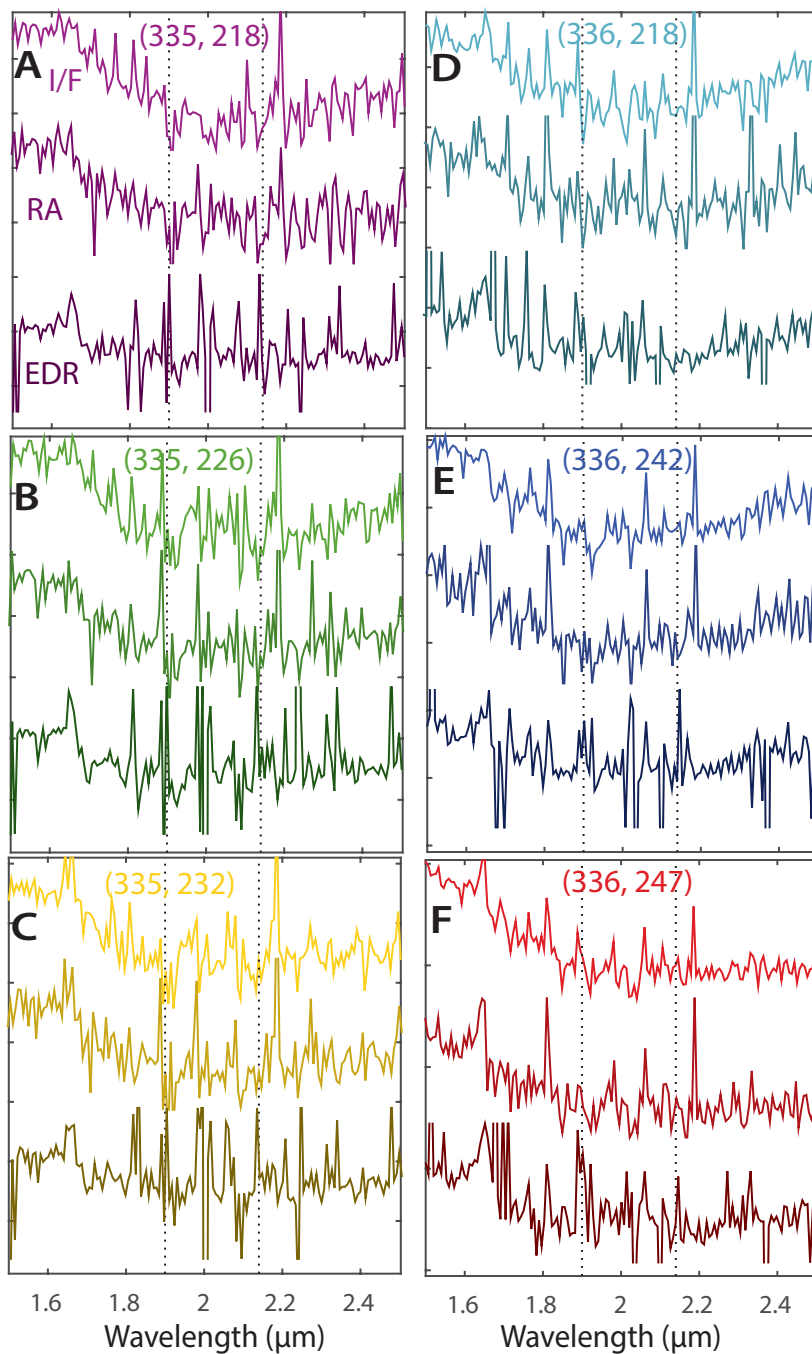
Ratioed I/F, RA, EDR spectra (offset) from RSLs in Palikir Crater (FRT0002038F)
