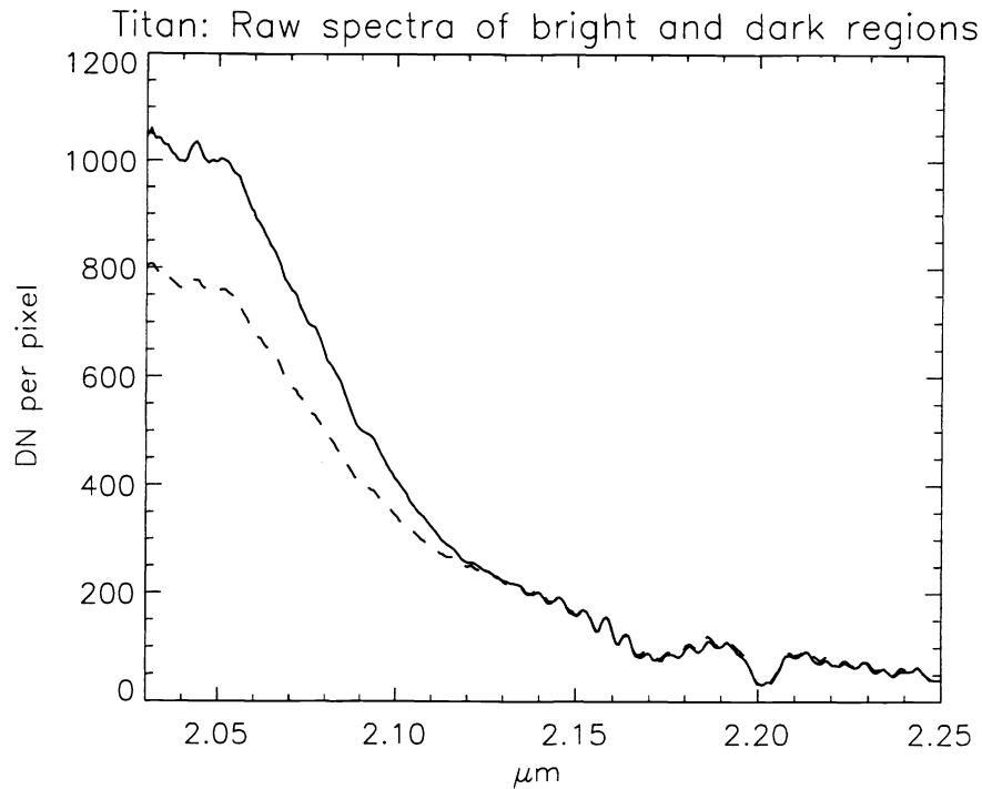
Figure 2. Sample raw K-band, R \sim 1000 , spectra for two positions on Titan's leading hemisphere. The upper curve is taken from the higher albedo region near the center of the leading hemisphere, while the lower curve is taken from a lower albedo region.
