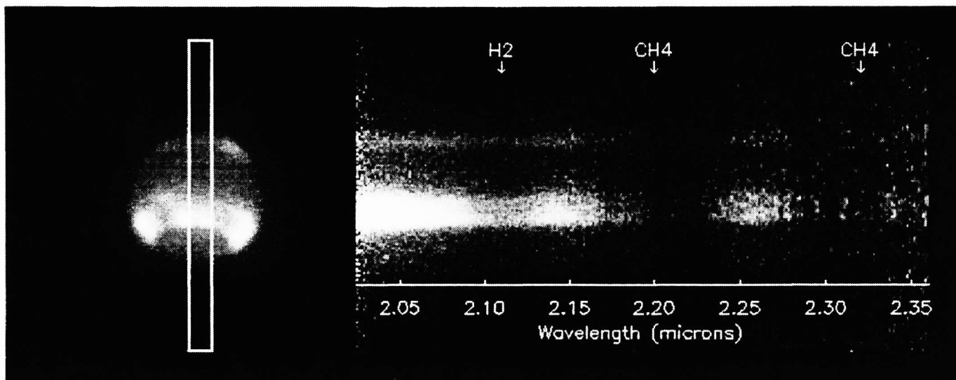
Figure 1. Neptune spectra (right) taken along a longitudinal slice of the AO-corrected disk (left).
