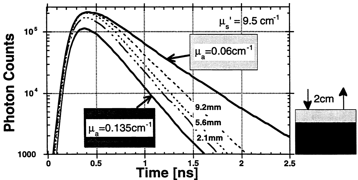
Fig.5: Experiments on layered gel phantoms with a layer of low absorbing gel on top of a high absorbing gel. The values labeled along the dashed curves indicate the thicknesses of the top layer.
