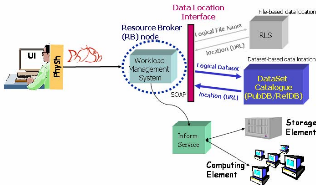
Fig. 1. Description of the analysis job submission in Grid. The user on the UI provides dataset and private code. The Workload Management System discovers the data location, via the Data Location interface to several catalogues, and submits the jobs on resources hosting the data.
