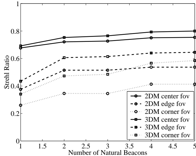
Figure 2. Strehl Ratio vs the number of natural beacons for the 2 and 3 DM sodium/natural hybrid configuration at the center, edge and corner of the field. The FOV is 148.148 \mu\text{rad} and the number of subapertures for the 5 sodium beacons and natural beacons are 12 \times 12 and 1 \times 1 respectively. Results at 1.65 \mu\text{m} are shown.
