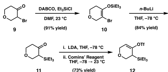
Scheme 1. Synthesis of silyl triflate 12 . DABCO=1,4-diazabicyclo[2.2.2]octane, DMF= N,N -dimethylformamide, THF=tetrahydrofuran, LDA=lithium diisopropylamide, Comins' Reagent= N -(5-Chloro-2-pyridyl)bis(trifluoromethanesulfonimide).
