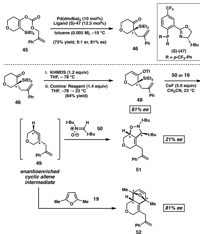
Scheme 2. Catalytic asymmetric approach and cycloaddition results. dmdba=3,5,3',5'-dimethoxydibenzylideneacetone, KHMDS=potassium bis(trimethylsilyl)amide, Comins' Reagent= N -(5-Chloro-2-pyridyl)bis(trifluoromethanesulfonimide), THF=tetrahydrofuran.
