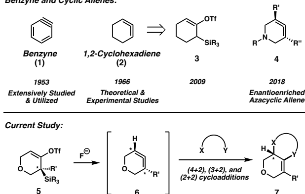
Figure 1. Highlights of benzyne and cyclic allene chemistry and cycloadditions of oxacyclic allenes described in this study. OTf=trifluoromethanesulfonate.
