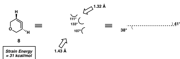
Figure 2. Ground state structure of oxacyclic allene 8 . The structure was computed using #B97XD/6-31G(d).
