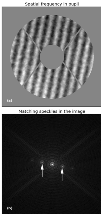
FIG. 2.— Illustration of the relation between sinusoidal modulation of the DM shape in the pupil and the resulting diffraction pattern in the image. In panel (a), one can approximately count 10 cycles of the sinusoid across the entire pupil. In the image (panel (b)), this modulation of the DM creates a pair of speckles (pointed by white arrows) located 10 \lambda/D away from the center of the field. These additional speckles interfere with the already present diffraction features such as rings, spikes and phase defects. They however do not interfere with incoherent structures like planets and disks.
