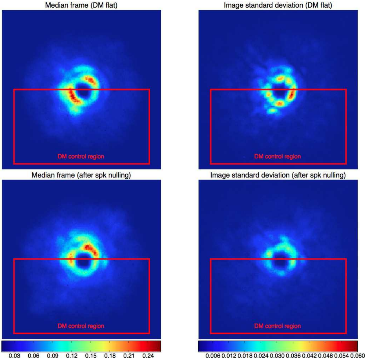
FIG. 4.— Statistical properties (median and standard deviation) of coronagraphic images acquired by HiCIAO for two SCExAO DM shapes. The top row is for a flat DM shape, that maximizes the Strehl ratio. The bottom row is for a DM shape resulting from a speckle nulling loop. The colorbar scale used for the images on the left (median) is calibrated in contrast.
