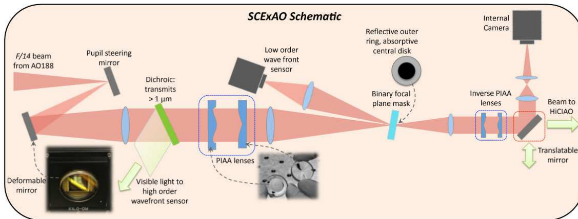
FIG. 1.— Schematic representation of the optics inside the SCEXAO IR coronagraph used to produce the results presented in this paper.
