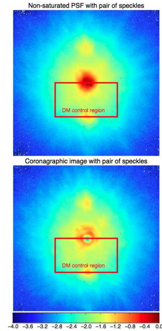
FIG. 3.— Comparison of a non-coronagraphic (top panel) and a coronagraphic (bottom panel) image acquired by HiCIAO behind SCExAO, with an added pair of speckles at max angular separation (log contrast scale). The red box highlights the area controlled by the DM during the experiments reported in this paper. Added speckles like these enable the calibration of the image in contrast, even if the central star is blocked by the coronagraph.
