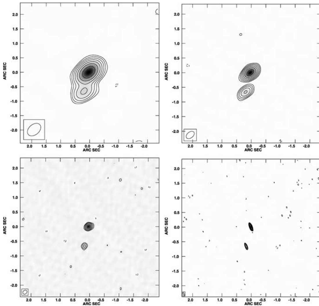
Figure 1. VLA and MERLIN maps of B0850+054. Top left: VLA 5-GHz map with a restoring beam of 524 \times 356 \text{ mas}^2 at a position angle of -49^\circ 9' . The data are uniformly weighted and the rms noise in the map is 157 \mu\text{Jy beam}^{-1} . Top right: VLA 8.5-GHz map with a restoring beam of 317 \times 200 \text{ mas}^2 at a position angle of -51^\circ 6' . The data are uniformly weighted and the rms noise in the map is 121 \mu\text{Jy beam}^{-1} . Bottom left: VLA 15-GHz map with a restoring beam of 153 \times 123 \text{ mas}^2 at a position angle of -46^\circ 2' . The data are uniformly weighted and the rms noise in the map is 288 \mu\text{Jy beam}^{-1} . Bottom right: MERLIN 5-GHz map with a restoring beam of 114 \times 38 \text{ mas}^2 at a position angle of 22^\circ 2' . The data are naturally weighted and the rms noise in the map is 100 \mu\text{Jy beam}^{-1} . All maps are plotted on the same angular scale and each has the restoring beam plotted in the bottom left-hand corner. Contours are plotted at multiples (-1, 1, 2, 4, 8, 16, \text{etc.}) of 3\sigma where \sigma is the off-source rms noise in the map. Image A is the northernmost of the two components.
