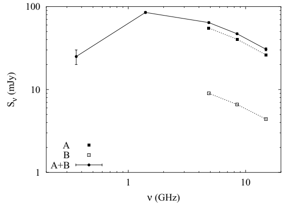
Figure 4. Radio spectrum of B0850+054. The solid line shows total flux densities (A+B) whilst below this the individual A and B flux densities are plotted where possible.
