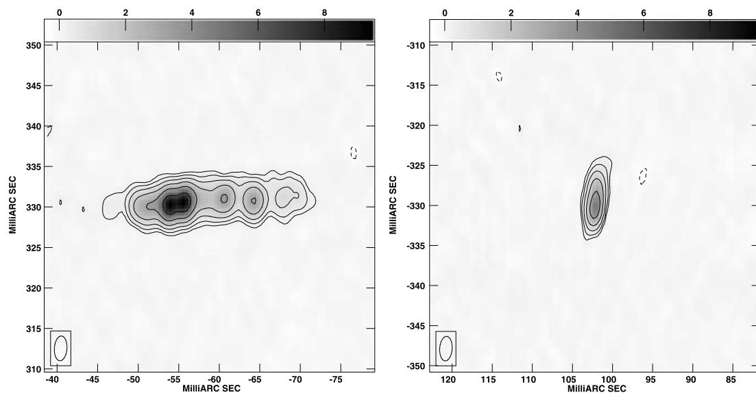
Figure 2. VLBA 5-GHz maps of image A (left) and image B (right) of B0850+054. The maps are uniformly weighted and both are plotted on the same angular scale. The restoring beam is shown in the bottom left-hand corner of each map and has a FWHM of 3.1 \times 1.6 \text{ mas}^2 at a position angle of -3^\circ 8' . Contours are plotted at multiples ( -1, 1, 2, 4, 8, 16 , etc.) of 3\sigma , where \sigma is the off-source rms noise in the map ( 50 \mu\text{Jy beam}^{-1} ). The grey-scale represents surface brightness in units of \text{mJy beam}^{-1} . Positions are offset from 08^{\text{h}}52^{\text{m}}53^{\text{s}}.5772, +5^\circ 15' 15''.329 (J2000).
