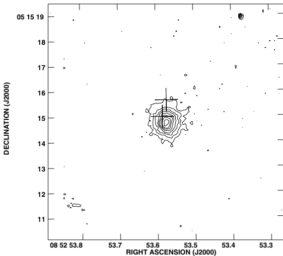
Figure 3. UKIRT K -band image of B0850+054. Contours are plotted at the background sky level plus linearly increasing multiples ( -1, 1, 2, 3 , etc.) of three times the off-source rms noise. The crosses mark the position of the A and B components.
