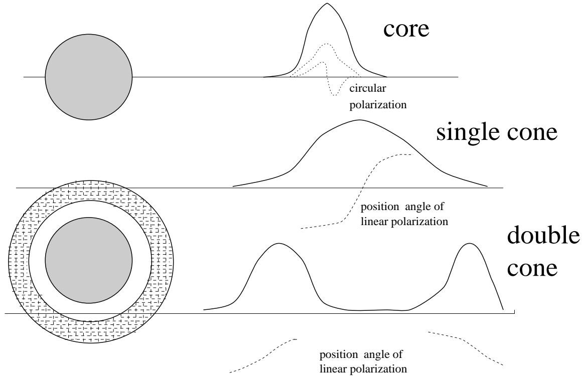
Fig. 2.— Example of emission geometry that produces core and cone profiles.
