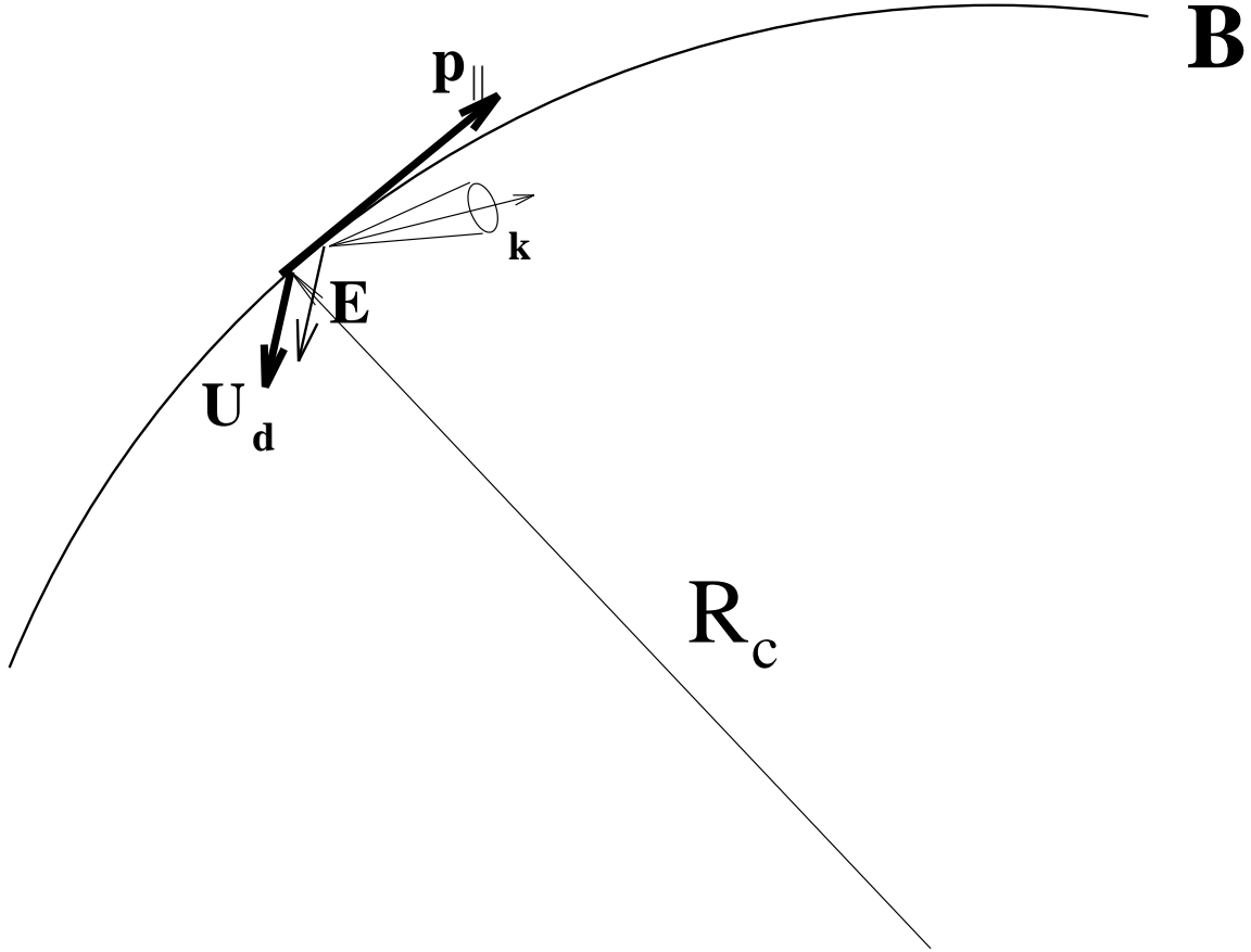
Fig. 4.— Cherenkov-drift emission. Drift velocity \mathbf{u}_d is perpendicular to the plane of the curved field line ( \mathbf{B} - \mathbf{R}_c ) plane, \mathbf{R}_c is a local radius of curvature). The emitted electromagnetic waves are polarized along \mathbf{u}_d . The emission is generated in the cone centered at the angle \theta^{em} = u_d/c and with the opening angle (2\delta)^{1/2} \ll \theta^{em} .
