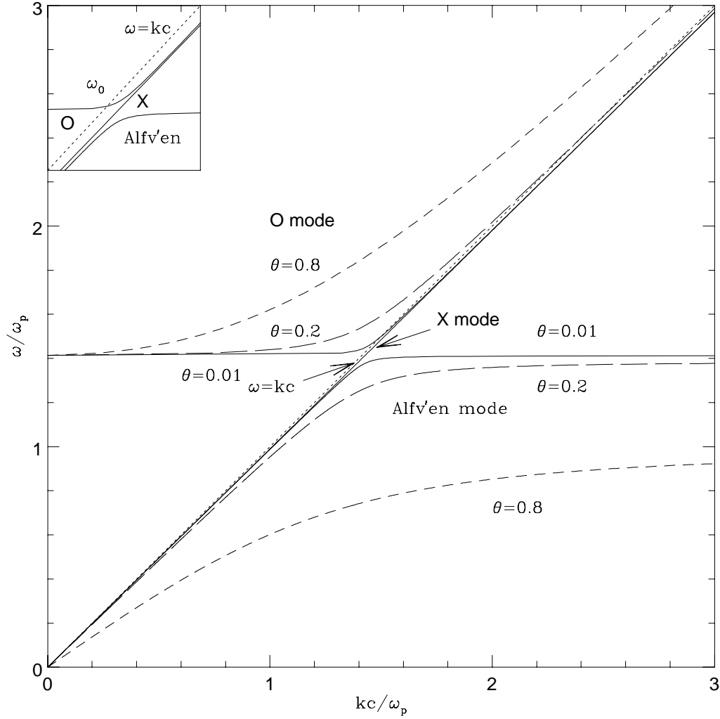
Fig. 5.— Dispersion curves for the waves in a cold electron-positron plasma in the plasma frame in the limit \omega_p \ll \omega_B . There are three modes represented by the dashed (ordinary mode), solid (extraordinary mode) and long dashed (Alfvén mode). The dotted line represents the vacuum dispersion relation. For the exact parallel propagation, the dispersion curves for the ordinary mode and Alfvén mode intersect. The insert in the upper left corner shows the region near the cross-over point \omega_0 .
