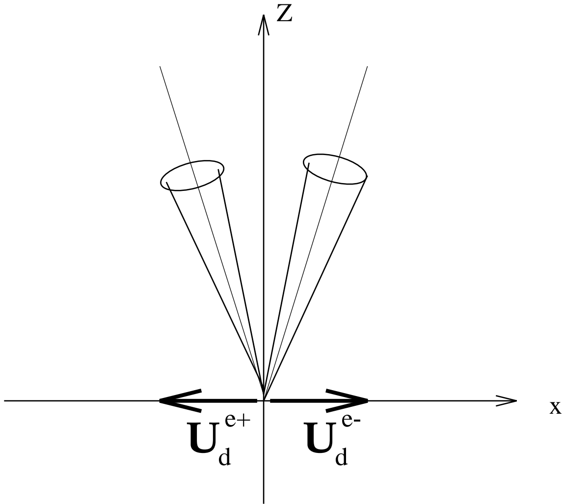
Fig. 9.— Switch of the sense of the circular polarization due to the cyclotron-Cherenkov resonance on the tail of the plasma distribution. The drift velocity of the electron and positron is in the opposite direction. As the line of sight crosses the emission region, the observer first will see the waves emitted by the particles of one sign of charge and then the other. The waves emitted by electron and positron have different circular polarization.
