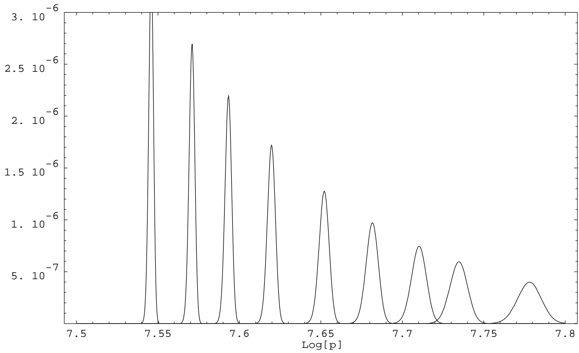
Fig. 10.— Evolution of the primary beam distribution function due the curvature radiation reaction. For the illustrative purposes we chose the initial beam \gamma -factor equal to 6 \times 10^7 , and the initial scatter in Lorentz factors \Delta\gamma = 10^6 .
