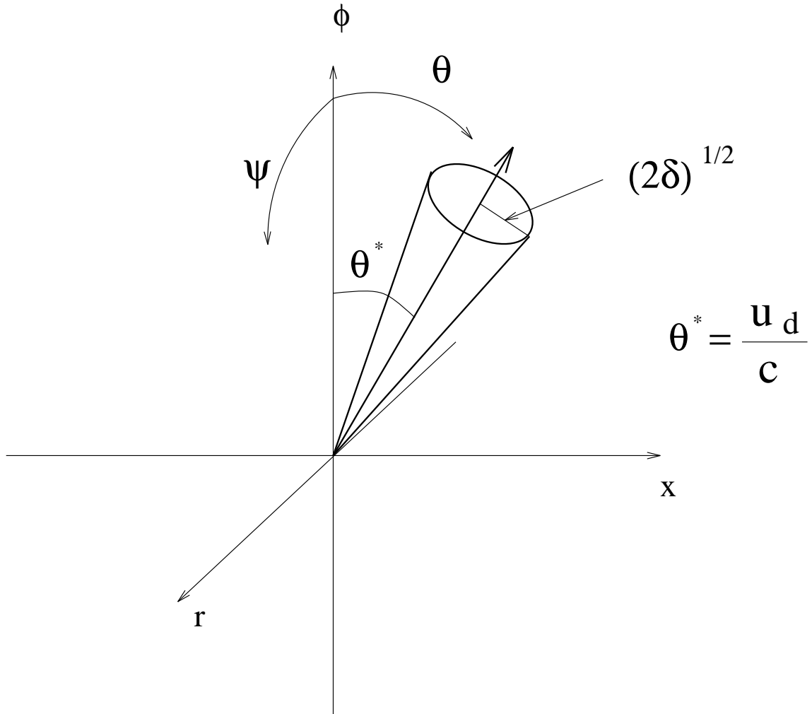
Fig. 7.— Emission geometry of the Cherenkov-drift resonance
