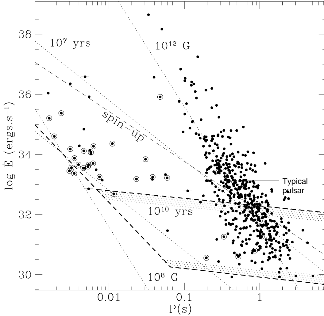
Fig. 3.— The dotted lines show constant spin down ages and magnetic fields. There is also a dashed line for the equilibrium period spin-up. The heavy dashed curves and shading illustrate several death lines from the literature (see Hansen 1997 for references). The circles indicate binary pulsars and those points with horizontal lines through them are in globular clusters with apparently negative \dot{E} (they are contaminated by cluster accelerations).
