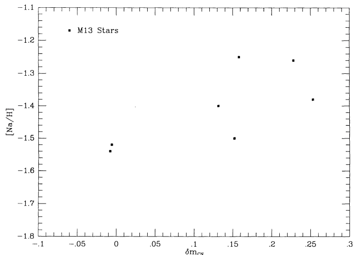
FIG. 8.—Sodium abundance vs. \delta m_{\text{CN}} from Suntzeff (1981). The correlation is good. This suggests that the source of the Na variation may be the same as that of the N variation.
