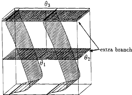
Figure 2: Extra Branch Singularities
