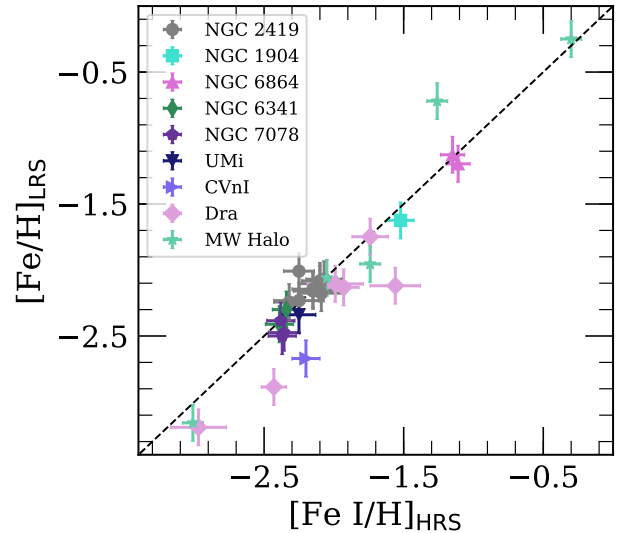
Figure 7. Metallicity measured from LRS ( [\text{Fe}/\text{H}]_{\text{LRS}} ) versus HRS ( [\text{Fe I}/\text{H}]_{\text{HRS}} ) for MW GCs, dSphs, and halo stars. Between LRS and HRS data sets, we have measurements in common for 30 stars. Although some scatter is present between data sets, [\text{Fe I}/\text{H}]_{\text{HRS}} and [\text{Fe}/\text{H}] are strongly correlated at high significance across multiple orders of magnitude in metallicity.
