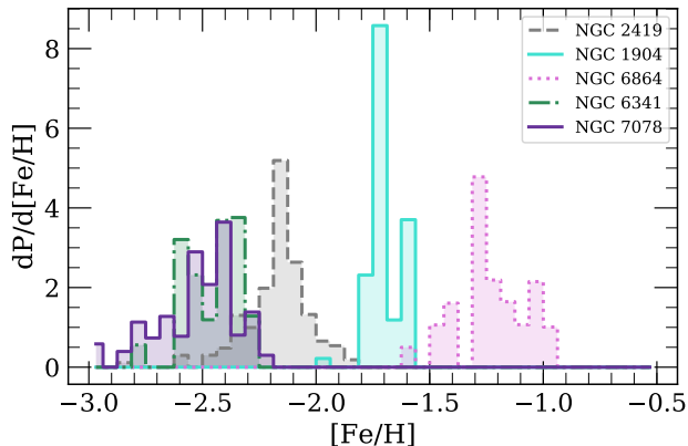
Figure 4. Error-weighted metallicity ( [\text{Fe}/\text{H}] ) distribution functions for RGB members of Galactic globular clusters NGC 2419 ( grey ), NGC 1904 ( cyan ), NGC 6864 ( magenta ), NGC 6341 ( green ), and NGC 7078 ( purple ). Only stars for which \delta[\text{Fe}/\text{H}] < 0.3 dex are shown. We find mean cluster metallicities of -2.14 dex, -1.70 dex, -1.22 dex, -2.45 dex, and -2.50 dex for the four respective clusters.
