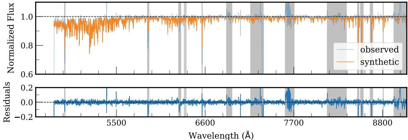
Figure 3. An example of a continuum-normalized observed spectrum ( light blue ) and its best-fit synthetic spectrum ( orange ). The observed spectrum corresponds to the same object in Figure 2. We show the entire fitted wavelength range ( \sim 4500 - 9100 \text{ \AA} ) for this object. The highlighted regions ( grey ) correspond to our standard mask (§ 3.4), which excludes lines such as H\beta , Na D1 and D2 from the fit. We adopt the parameters of the best-fit synthetic spectrum for the observed spectrum, T_{\text{eff}} = 4300 \text{ K} , \log g = 0.71 \text{ dex} , [\text{Fe}/\text{H}] = -2.07 \text{ dex} , [\alpha/\text{Fe}] = 0.29 \text{ dex} , and \Delta\lambda = 2.60 \text{ \AA FWHM} . We measure \chi^2_{\nu} = 1.63 for the quality of the fit across the full wavelength range, based on the regions of the spectrum used to measure [\text{Fe}/\text{H}] (§ 4.4). The normalized residuals ( dark blue ) between the continuum-refined observed spectrum and best-fit synthetic spectrum are also shown. The residuals have been scaled by the inverse variance of the observed spectrum and the degree of freedom of the fit, such that each pixel represents the direct contribution to \chi^2_{\nu} .
