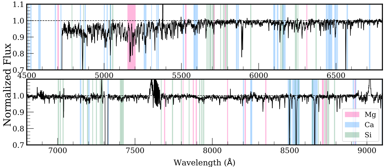
Figure 2. Wavelength regions sensitive to changes in [\alpha/\text{Fe}] for the spectral resolution of the DEIMOS 600ZD grating ( \sim 2.8 \text{ \AA} ). We show an example spectrum ( black ) over the wavelength range 4500–9100 \text{\AA} , where we corrected the spectrum for telluric absorption (§ 3.1) and performed an initial continuum normalization (§ 3.3). We do not show spectral regions with wavelengths below 4500 \text{\AA} , since low S/N generally prevents utilization of the observed spectrum in this wavelength range. The spectrum is for a star in the globular cluster NGC 2419. Spectral regions sensitive to Mg, Ca, and Si are shown as highlighted ranges in magenta, blue, and green respectively. The atmospheric value of [\alpha/\text{Fe}] is measured using the union of the Mg, Ca, and Si spectral regions.
