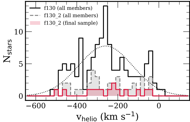
Figure 12. Heliocentric velocity histogram for the final 11 star sample drawn from f130_2 ( red ) compared to the distributions for all 37 M31 RGB stars in f130_2 ( grey ) with successful radial velocity measurements. We also show the velocity histogram for 128 M31 RGB stars ( black ) from the broader sample of nearby fields, including f130_2, known as f130 (Gilbert et al. 2007). The dotted line is the best-fit Gaussian ( \bar{v} = -260 \text{ km s}^{-1} , \sigma_v = 132 \text{ km s}^{-1} ; Gilbert et al. 2007) to f130, which corresponds to a kinematically hot spheroid component with no detected substructure (i.e., the smooth stellar halo of M31). We find that our final sample is consistent with the kinematics of the hot spheroid.
