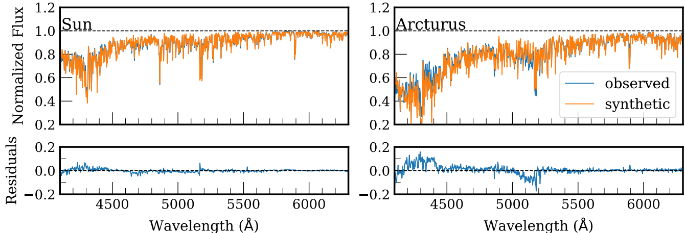
Figure 1. (Top) A comparison between high-resolution spectra (Hinkle et al. 2000) (blue) of the Sun (left) and Arcturus (right) and synthetic spectra (orange) generated using the blue line list (§ 4.1). Both spectra are smoothed to the expected resolution of the DEIMOS 600ZD grating ( \sim 2.8 \text{ \AA} ). For a description of synthetic spectrum generation, see § 4.2. (Bottom) The difference between the observed and synthetic spectra for the Sun and Arcturus. To improve the agreement between the synthetic and observed spectra, we have manually vetted the line list, adjusting the oscillator strengths of discrepant atomic transitions as necessary. In this process, we have favored the Sun over Arcturus, thus the larger residuals between the observed and synthetic spectra for the latter star (which has a lower effective temperature).
