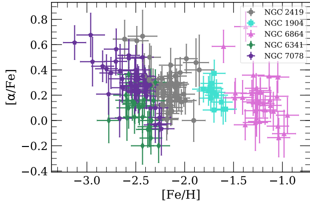
Figure 6. Atmospheric [\alpha/\text{Fe}] versus [\text{Fe}/\text{H}] for the same data set as Figure 4, where we also exclude points with \delta([\alpha/\text{Fe}]) > 0.3 dex. There is no apparent anticorrelation between [\alpha/\text{Fe}] and [\text{Fe}/\text{H}] within a GC, indicating that our method does not show any unphysical covariance between these two parameters.
