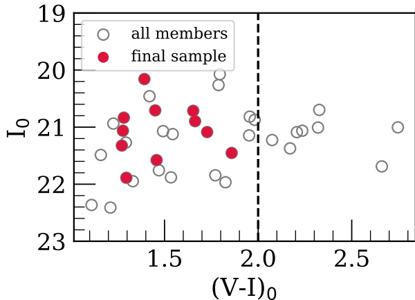
Figure 11. (I, V-I) color-magnitude diagram for M31 RGB stars from a 23 kpc field (f130_2) with no identified substructure. We show both stars contained in the final sample ( red filled circles ) (§ 8.2) and the full sample of member stars ( grey open circles ). The dashed vertical line represents a rough threshold in color above which stars are likely to show evidence for strong TiO absorption in their spectra ( (V-I)_0 > 2.0 ). The final sample of stars shows significant overlap with the full distribution of M31 members, aside from known color biases that we have introduced in our sample selection.
