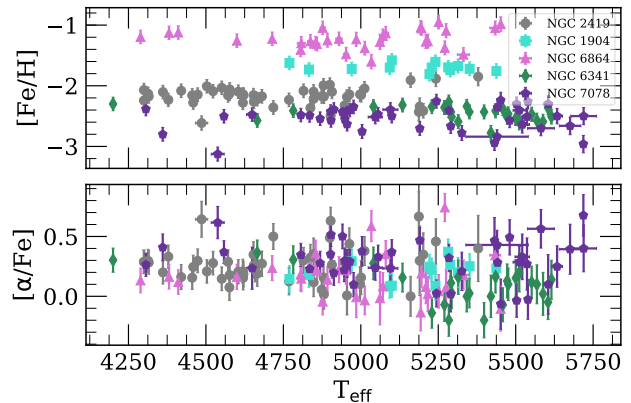
Figure 5. ( Top ) metallicity ( [\text{Fe}/\text{H}] ) and ( bottom ) [\alpha/\text{Fe}] vs. spectroscopic effective temperature ( T_{\text{eff}} ). We show only stars with \delta[\text{Fe}/\text{H}] < 0.3 dex and \delta[\alpha/\text{Fe}] < 0.3 dex in each panel. The lack of a trend between both [\text{Fe}/\text{H}] and [\alpha/\text{Fe}] with respect to T_{\text{eff}} for each GC implies that our chemical abundance analysis is robust to systematic covariance in these parameters.
