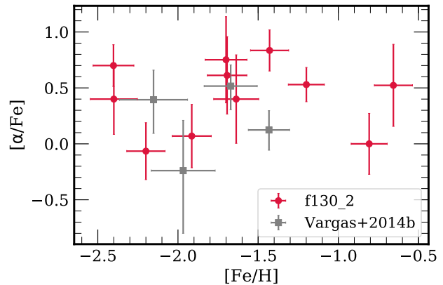
Figure 14. [\alpha/\text{Fe}] vs. [\text{Fe}/\text{H}] , measured from LRS, for M31 RGB stars (red circles) in the 23 kpc field. We show a subset of our entire sample, with \delta([\text{Fe}/\text{H}]) < 0.5 dex and \delta([\alpha/\text{Fe}]) < 0.5 dex, considering only stars with reliable abundance measurements. In total, we present [\alpha/\text{Fe}] measurements for 11 M31 halo stars, increasing the previous sample size of 4 stars (Vargas et al. 2014b). We plot the latter sample of metal-poor halo stars (grey squares) ( S/N \gtrsim 15 \text{ \AA}^{-1} ) over our data set for comparison ( S/N \sim 10-30 \text{ \AA}^{-1} ).
