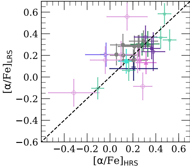
Figure 8. [\alpha/\text{Fe}]_{\text{HRS}} versus [\alpha/\text{Fe}]_{\text{LRS}} for the same data set as Fig. 7. We construct [\alpha/\text{Fe}]_{\text{HRS}} based on a weighting (§ 6.2) of its individual \alpha -element abundances. Open symbols indicate values of [\alpha/\text{Fe}]_{\text{HRS}} constructed from two or fewer individual \alpha -element abundance ratios. The LRS and HRS abundances exhibit broad agreement and show a clear correlation, despite the intrinsic differences between the sets of measurements.
