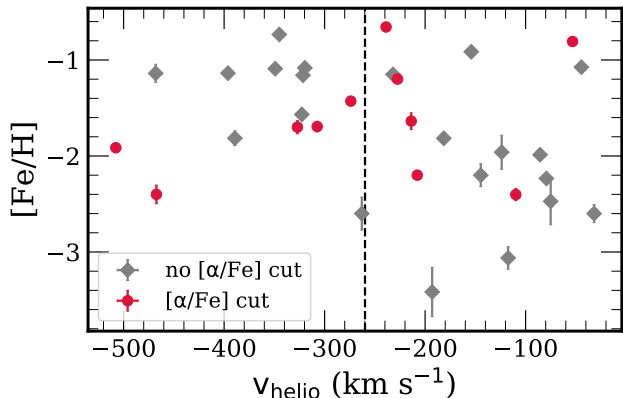
Figure 13. Spectroscopic metallicity ( [\text{Fe}/\text{H}] ) as a function of heliocentric velocity for M31 RGB stars in f130_2. The typical uncertainty in velocity ( \sim 3.5 \text{ km s}^{-1} ) is smaller than the size of the data points. In addition to our final sample ( red circles ), which contains only reliable [\alpha/\text{Fe}] measurements (§ 8.2), we show a broader sample ( grey diamonds ) that contains well-constrained [\text{Fe}/\text{H}] measurements, with no cuts on [\alpha/\text{Fe}] . No apparent correlation exists between radial velocity and metallicity in the field, where our final sample is representative of the broader sample.
