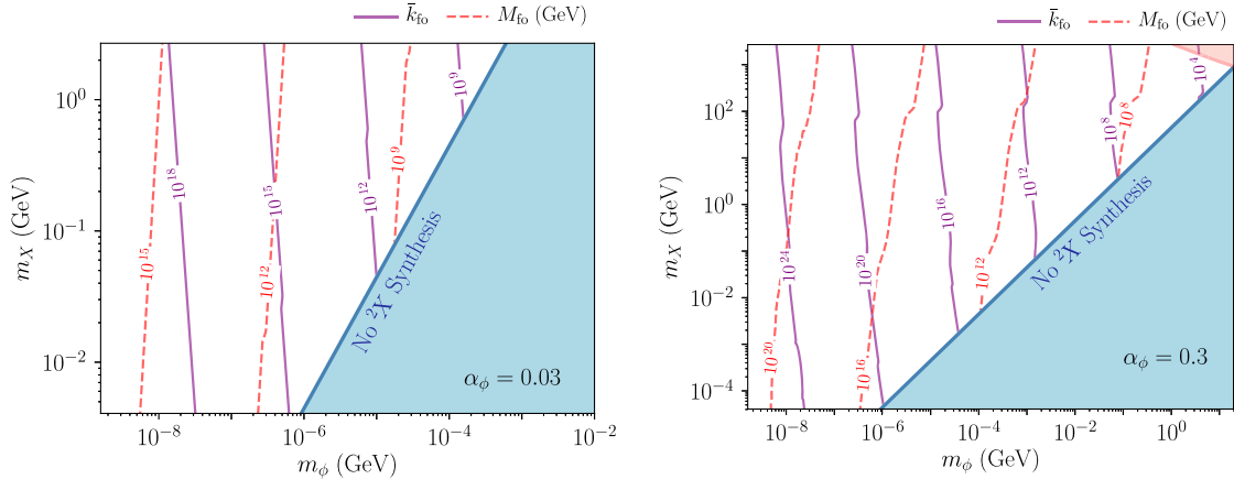
FIG. 2. Contours of typical nugget number exiting big bang darkleosynthesis, \bar{k}_{\text{fo}} (dashed red line) and typical nugget mass \bar{M}_{\text{fo}} (solid purple) for \alpha_\phi = 0.03 (left) and \alpha_\phi = 0.3 (right). The temperature of the dark sector is assumed to be roughly T_X \approx T_\gamma . The blue shaded region corresponds to \text{BE}_2 < m_\phi , where {}^2X synthesis will not be efficient [Eq. (5)]. The upper m_X cutoff corresponds to the requirement that the {}^2X fusion rate be smaller than Hubble as in Eq. (6), and the lower m_X cutoff corresponds to T_{\text{synth}} \lesssim 10T_{\text{eq}} . (See Fig. 1.) The various kinks in the contours are results of the change in g_* as the synthesis temperature passes through the QCD phase transition and neutrino decoupling.
