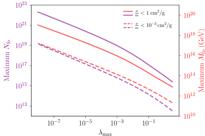
FIG. 1. Maximum achievable nugget size N_{\text{fo}} (purple) and nugget mass M_{\text{fo}} (red) as a function of the maximum scalar force mediator quartic coupling \lambda_{\text{max}} . Given a conservative constraint on late-universe DM nugget interaction cross sections \sigma_{\text{DM}}/m_{\text{DM}} \lesssim 1 \text{ cm}^2/\text{g} (solid) or \sigma_{\text{DM}}/m_{\text{DM}} \lesssim 10^{-3} \text{ cm}^2/\text{g} (dashed), maximum possible sizes are realized when only a scalar mediator contributes to large nugget properties (i.e. when effects of a vector mediator are negligible). \lambda_{\text{max}} serves as a measure of fine tuning for achieving large nuggets, as radiative corrections tend to drive \lambda to be relatively large. The synthesis temperature is (conservatively) taken to be T_{\text{syn}} = (m_X - \bar{m}_X)/15 —the maximum possible 2-body binding energy times a typical Boltzmann suppression factor, 1/30 . A typical model is expected to have lower synthesis temperature and therefore smaller freeze-out sizes and masses.
