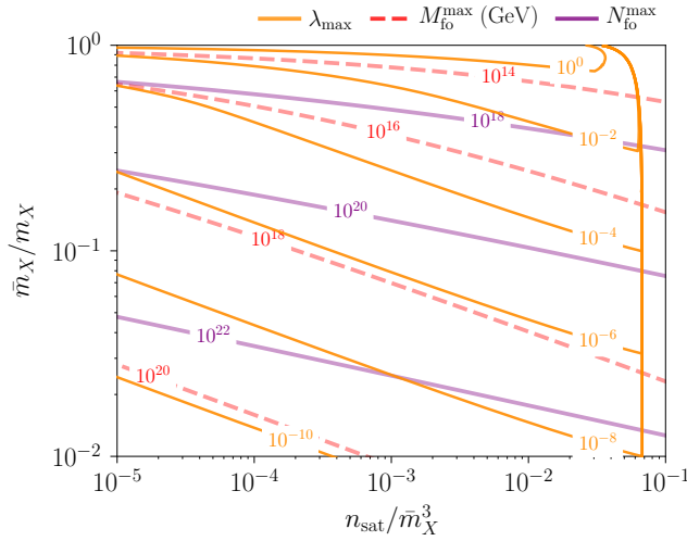
FIG. 3. Available physical parameter space (n_{\text{sat}}/\bar{m}_X^3, \bar{m}_X/m_X) for an extended nuclear model as described in Sec. II with V(\phi) = \frac{g_\phi^4}{3\pi^2} \lambda \phi^4 . The orange boundaries indicate the maximal allowed value for \lambda , which indicates fine-tuning. [See Eqs. (6), (8) and surrounding discussion.] The dashed red (solid purple) shows the maximum achievable typical freeze-out nugget mass (number of constituents) M_{\text{fo}} ( N_{\text{fo}} ) given \sigma_{\text{DM}}/m_{\text{DM}} \lesssim 1\text{cm}^2/\text{g} in the late Universe. [See Eqs. (23)-(22).] The synthesis temperature is (conservatively) taken to be T_{\text{syn}} = (m_X - \bar{m}_X)/15 . A typical model is expected to have lower synthesis temperature and to require lower \sigma_{\text{DM}}/m_{\text{DM}} to accord with galactic structure observations and therefore smaller nugget freeze-out sizes and masses.
