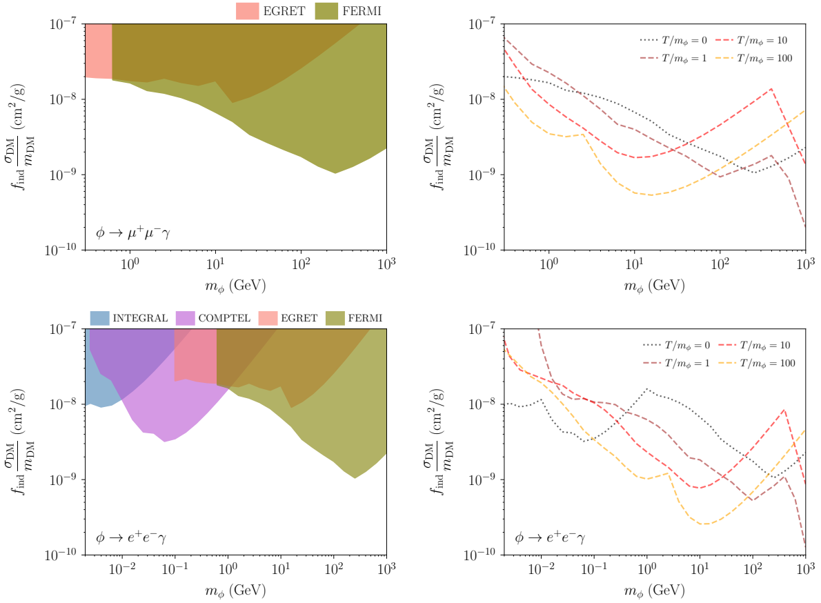
FIG. 6. Indirect detection constraints for a scalar mediator decaying into \phi \rightarrow \mu^+\mu^-\gamma (top) and \phi \rightarrow e^+e^-\gamma (bottom). Left : Constraints for nonrelativistic emissions, where the emitted mediators are assumed to be at rest. Right : Constraints for relativistic emissions, where the momentum of the mediator is assumed to follow a Boltzmann distribution.
