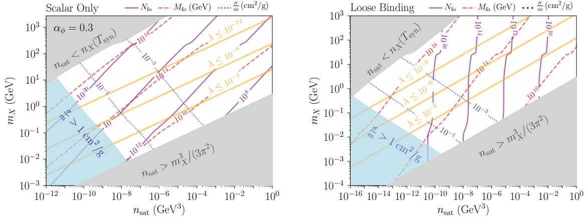
FIG. 5. Nugget size constraints for a scalar-binding model [left] and a benchmark loose-binding model ( \bar{m}_X = 0.9 m_X ) [right], when no bottleneck is present. The dashed red (solid purple) contours indicate the characteristic mass (size) of the nuggets exiting synthesis, where T_{\text{syn}} = \text{BE}_2/30 = \alpha_\phi^2 m_X/120 in the left panel and T_{\text{syn}} = m_X/150 in the right panel. The light blue regions are excluded by the SIDM constraint \sigma_{\text{DM}}/m_{\text{DM}} < 1 \text{ cm}^2/\text{g} . The dotted blue line shows contours of \sigma_{\text{DM}}/m_{\text{DM}} \sim 10^{-1} and 10^{-3} \text{ cm}^2/\text{g} , indicating possible formation of a collapsed galaxy core. The solid orange curves indicate the maximum allowed scalar quartic coupling \lambda for given m_X and n_{\text{sat}} . In order to reach regions of larger m_X at fixed n_{\text{sat}} , \lambda must be progressively smaller. Small \lambda values may imply fine-tuning. [See Eqs. (6), (8) and surrounding discussion.]
