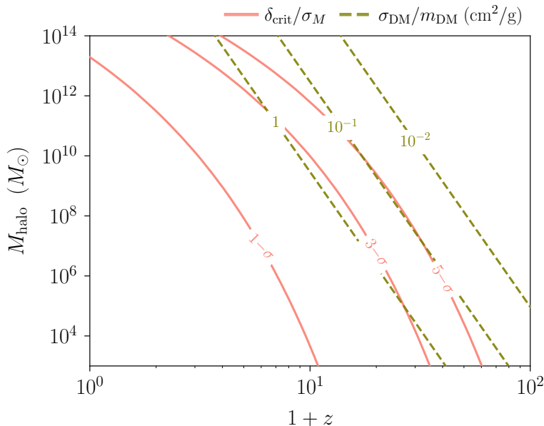
FIG. 7. Solid Red: contours of the halo mass ( M_{\text{halo}} ) vs red-shift ( 1+z ) that correspond to n - \sigma fluctuations in the Press-Schechter model. Dashed Green: regions with cooling timescale of order H_0^{-1} assuming \sigma_{\text{DM}}/m_{\text{DM}} \sim (1, 10^{-1}, 10^{-2}) \text{ cm}^2/\text{g}
