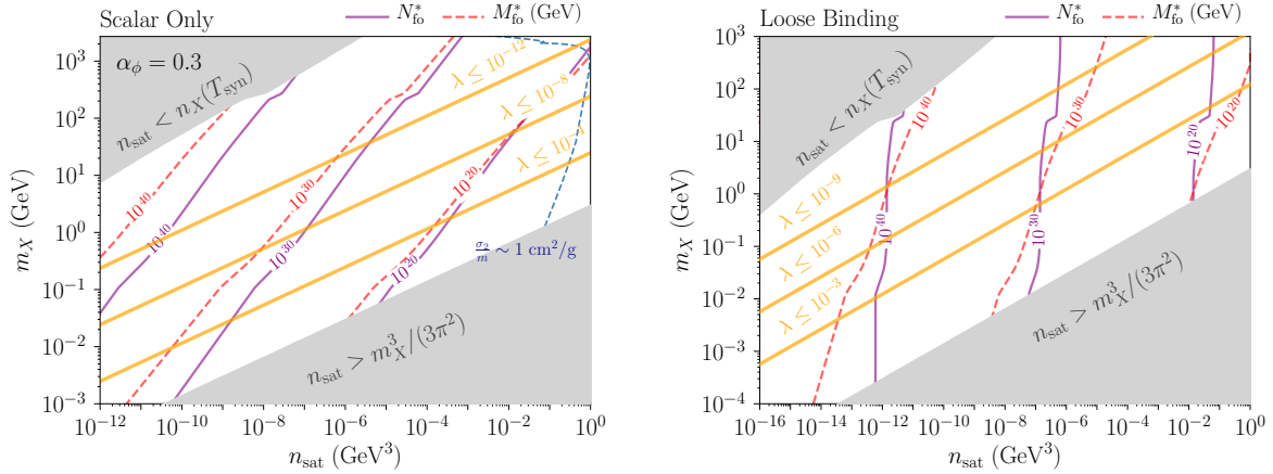
FIG. 8. Nugget size constraints for a scalar-binding model [left] and a benchmark loose-binding model ( \bar{m}_X = 0.9 m_X ) [right], when a bottleneck is present. The dashed red (solid purple) contours indicate the characteristic mass (size) of the nuggets exiting synthesis, where T_{\text{syn}} = \text{BE}_2/30 = \alpha_\phi^2 m_X/120 in the left panel and T_{\text{syn}} = m_X/150 in the right panel. Left : The region left of the dashed blue line is excluded by the SIDM constraint \sigma_{\text{DM}}/m_{\text{DM}} < 1 \text{ cm}^2/\text{g} assuming that the dominant form of DM (by mass) is {}^2X . Right : A similar SIDM curve is not shown as it is strongly model dependent. On both plots, the solid orange curves indicate contours of constant scalar quartic. Small \lambda values may imply fine-tuning. [See Eqs. (6), (8) and surrounding discussion.] It is possible to evade all SIDM constraints if synthesis ends when all small nuggets are depleted, in which case N_{\text{fo}}^* \sim p^{-1} as described in Eq. (42). For scenarios where p (the probability to pass the bottleneck) is large enough such that small nuggets are quickly depleted and fusion is quickly dominated by large nuggets fusion, the standard analysis in Sec. II C applies, and we refer to Fig. 5 for the relevant parameter space.
