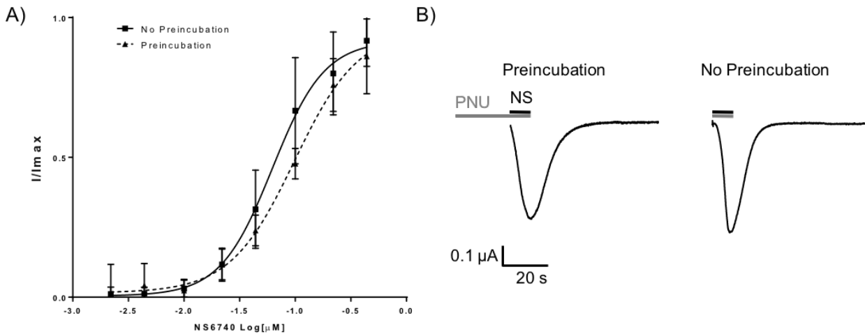
Fig. S1. Effect of pre-incubation with PAM PNU-120596 on NS6740 response. A) Shows EC_{50} curves with and without preincubation. B) Shows representative traces with and without preincubation.
