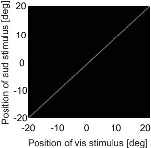
Forced fusion
