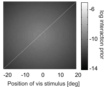
Causal inference
